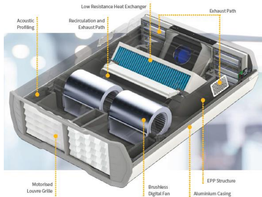
Figure 1 - Monodraught HVR Zero Hybrid ventilation unit
