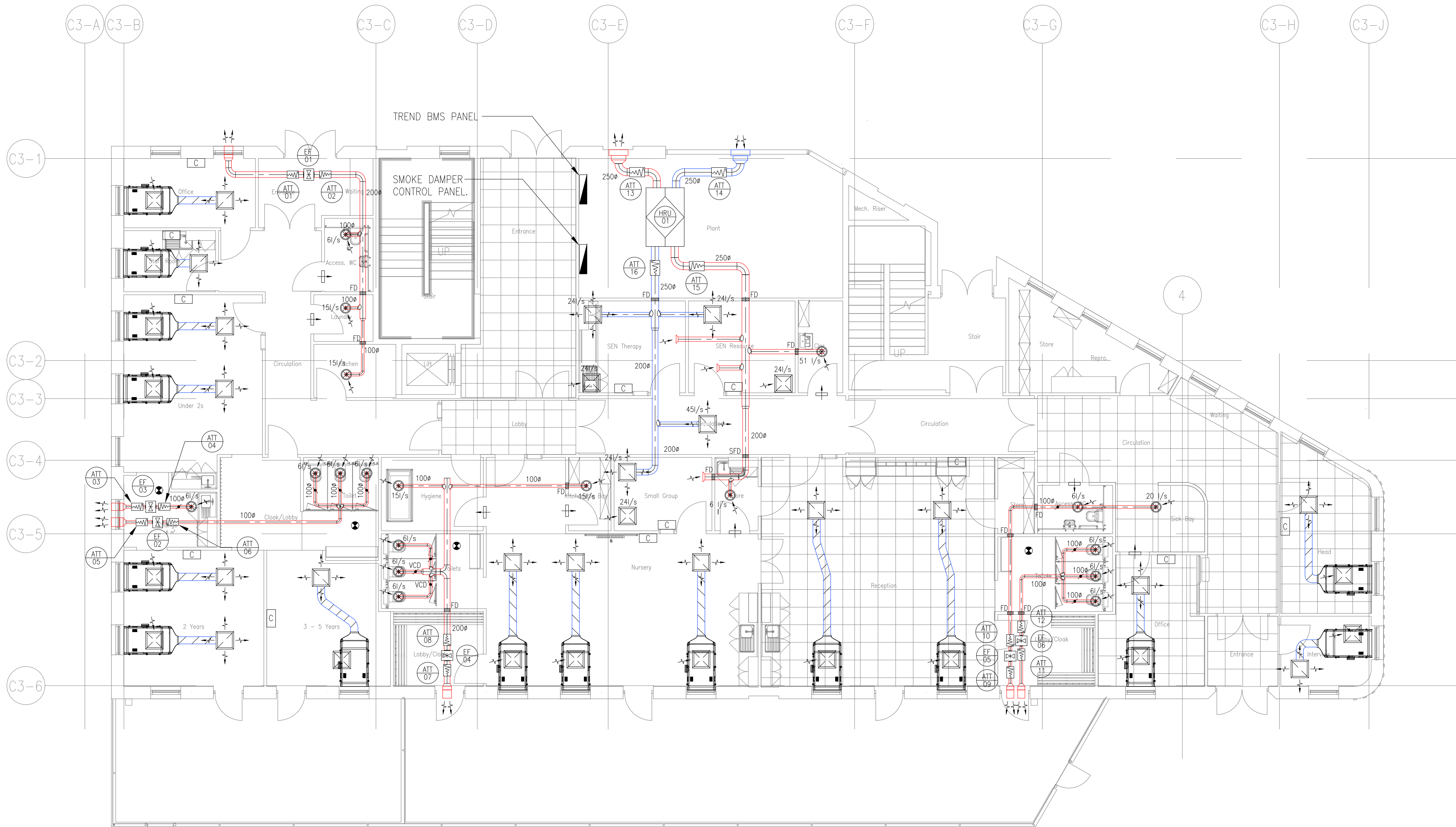
C3 - SCHOOL LEVEL 00 BASED ON C3 Primary School Architectural Model_Ver2_P03-Floor Plan - 00 - Ground Floor
