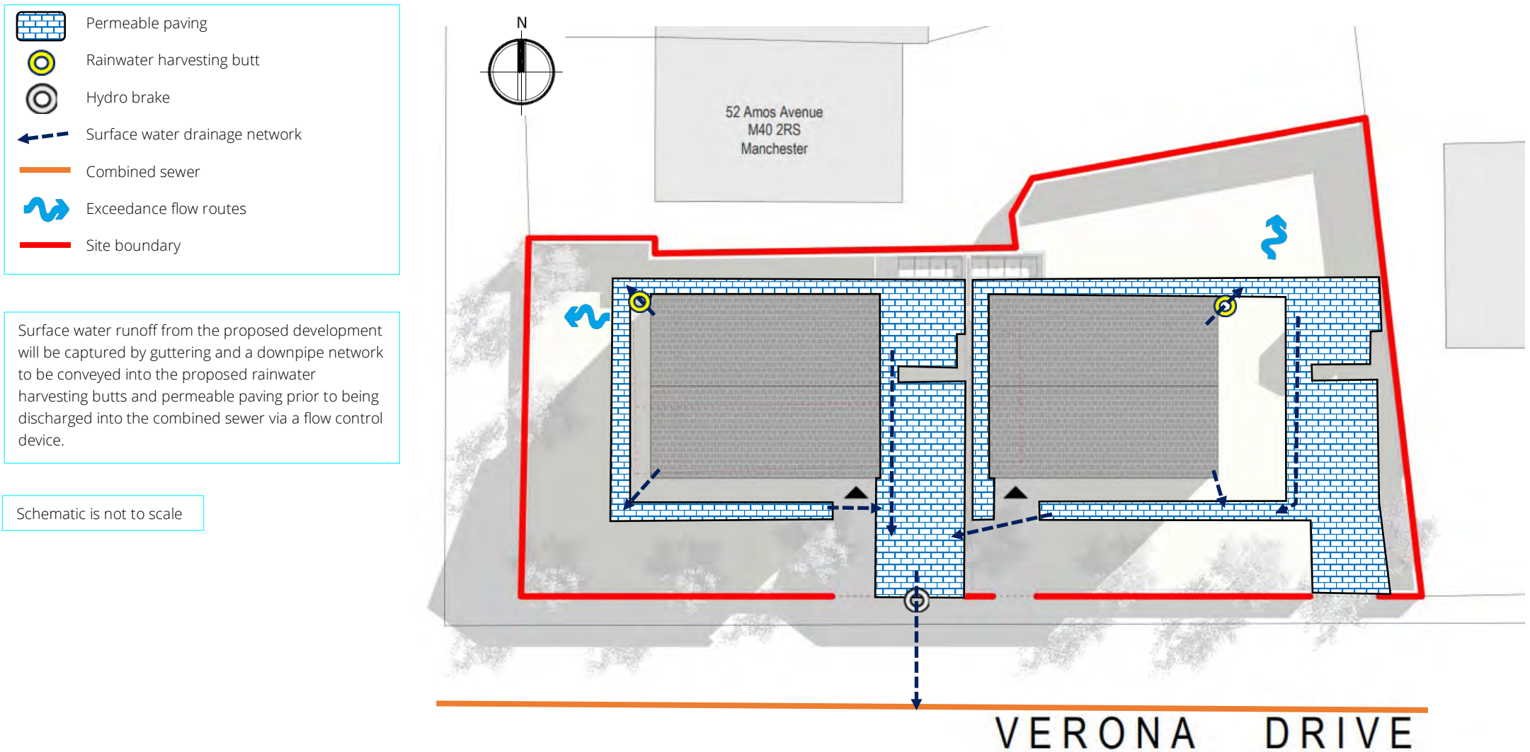
Figure 1. Proposed SuDS scheme layout
