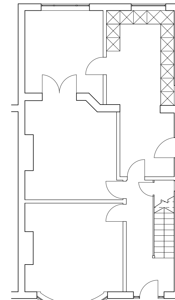
GROUND FLOOR SCALE 1:100 UID - E003
