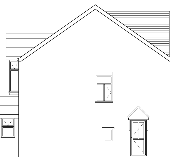
SOUTH ELEVATION SCALE 1:100 UID - P008
