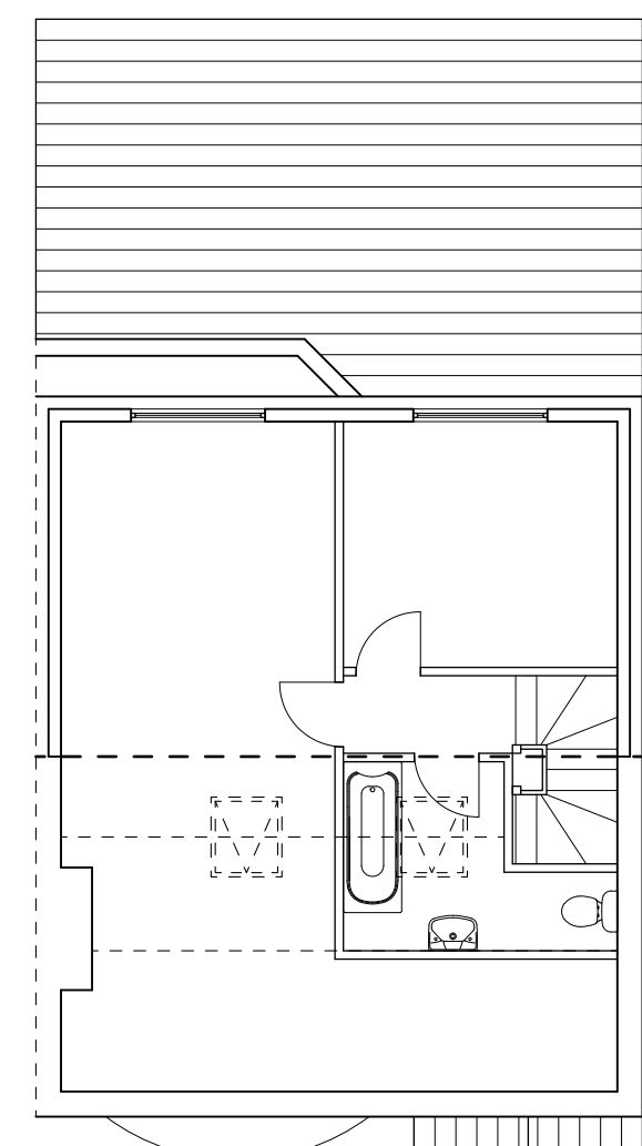
SECOND FLOOR SCALE 1:100 UID - P005
