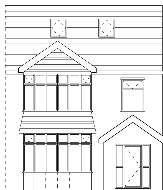
WEST ELEVATION SCALE 1:100 UID - P006
