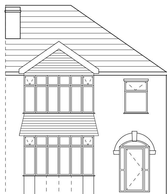
WEST ELEVATION SCALE 1:100 UID - E006
