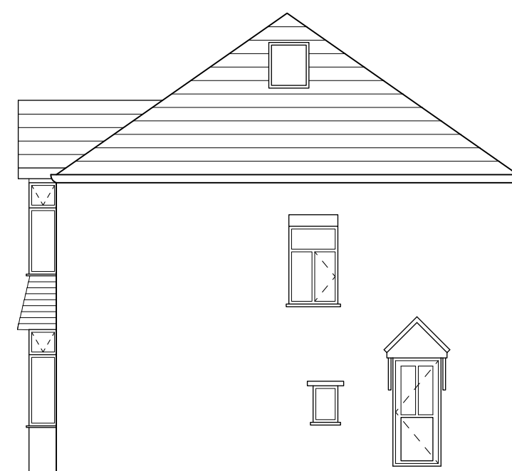
SOUTH ELEVATION SCALE 1:100 UID - E008
