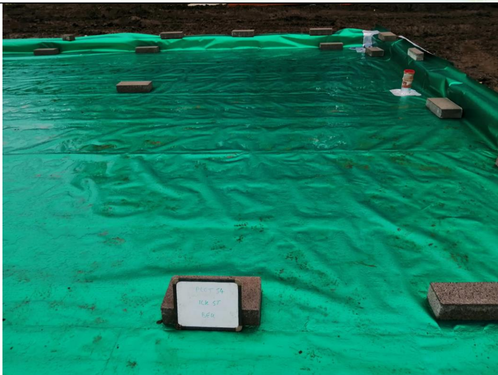
Photograph 4: Validation of Gas Membrane Installation
