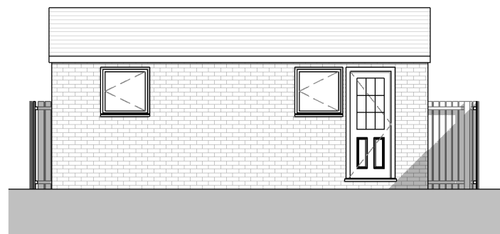
2 Front Elevation 1 : 100
