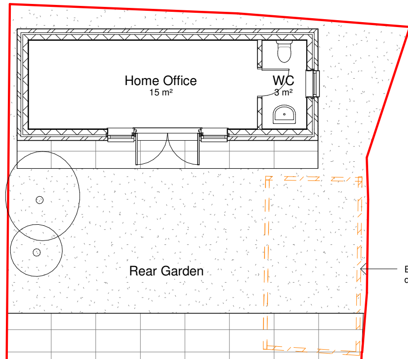
1 Proposed Rear Outbuilding 1 : 100
