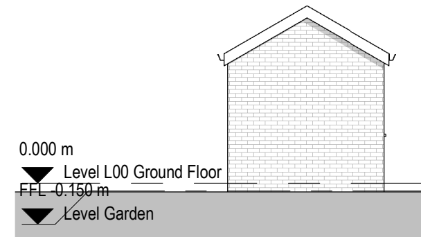
4 Outbuilding West Elevation 1 : 100
