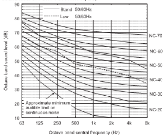
Sound level of PURY-P500YNW-A(-BS)
