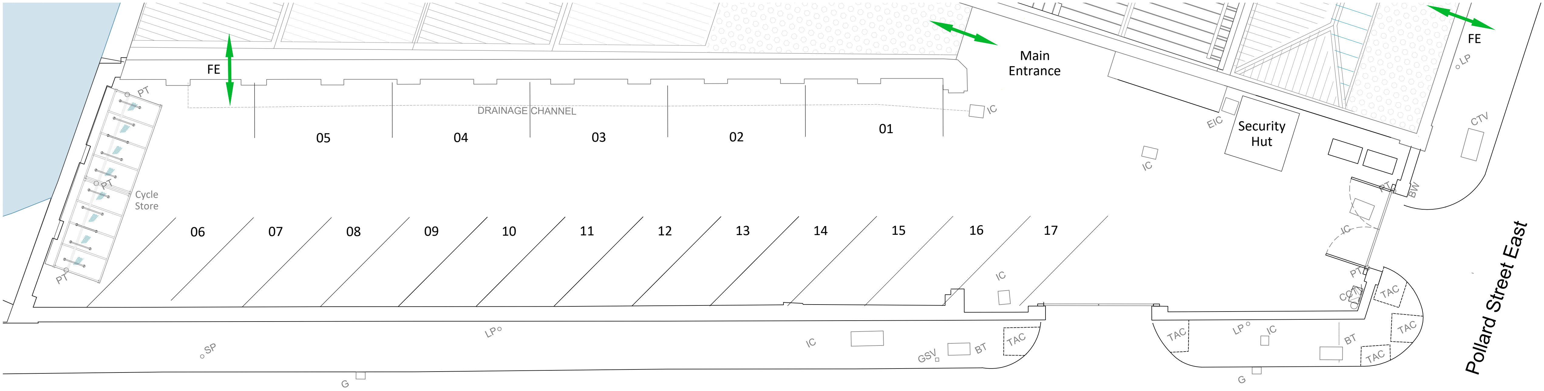
Existing Parking Plan Scale 1:100 0m 2m 4m 6m 8m 10m Scale Bar 1:100 @ A1
