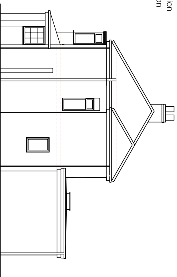
PROPOSED EXTENSION SIDE ELEVATION
