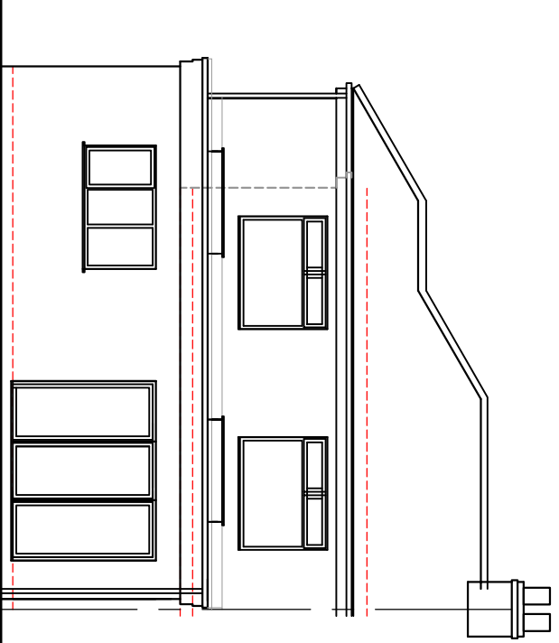
PROPOSED EXTENSION REAR ELEVATION
