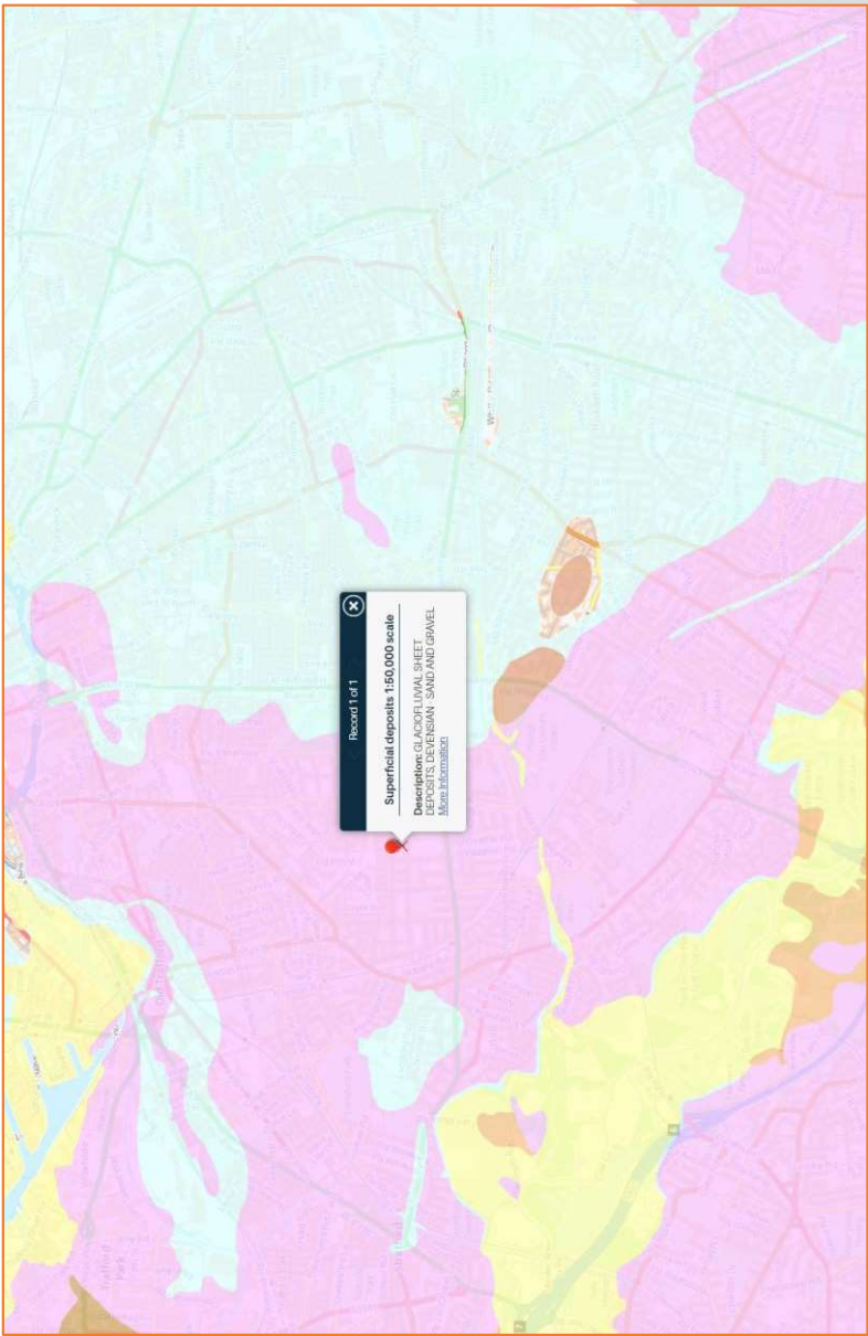
Figure 4: Local Superficial deposits geology (Source: BGS)
