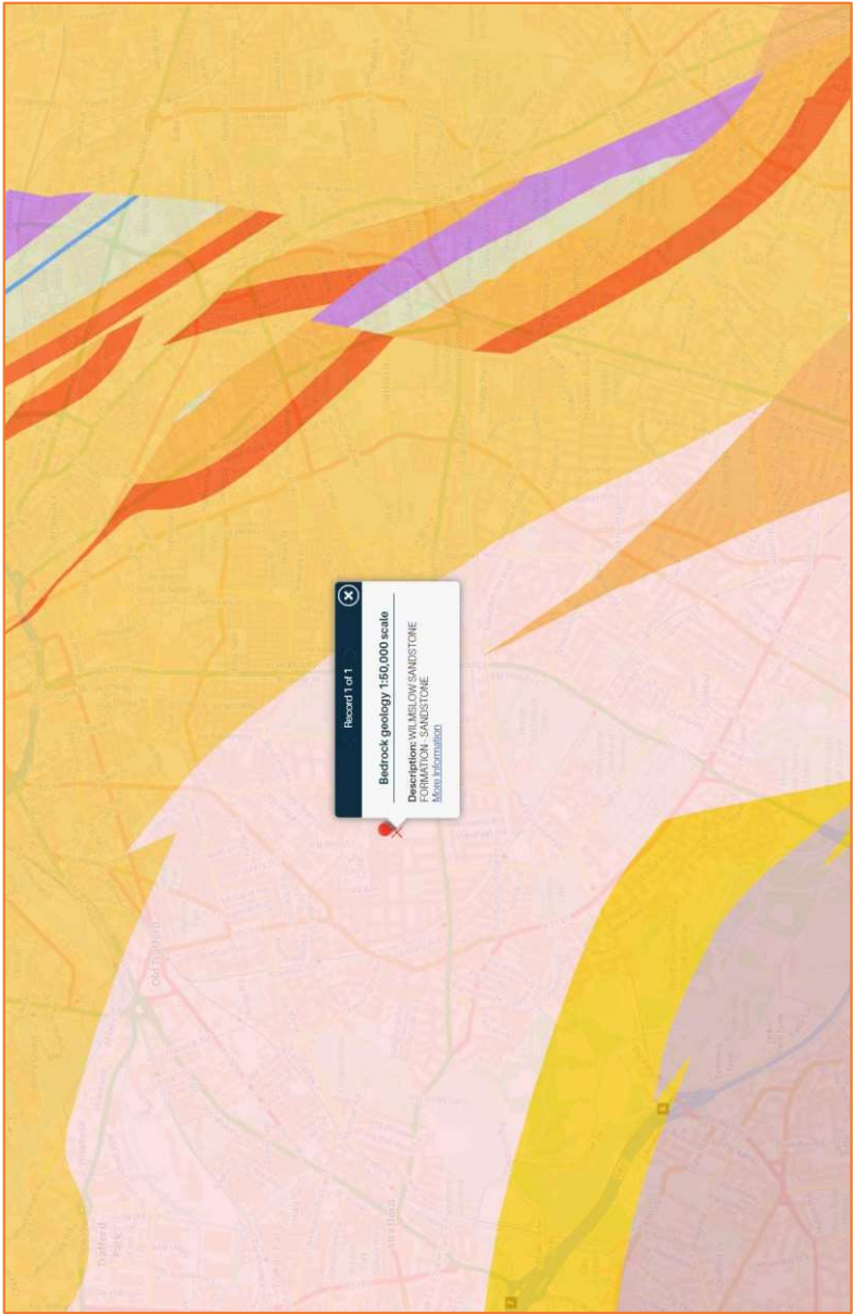
Figure 3: Local bedrock geology (Source: BGS)
