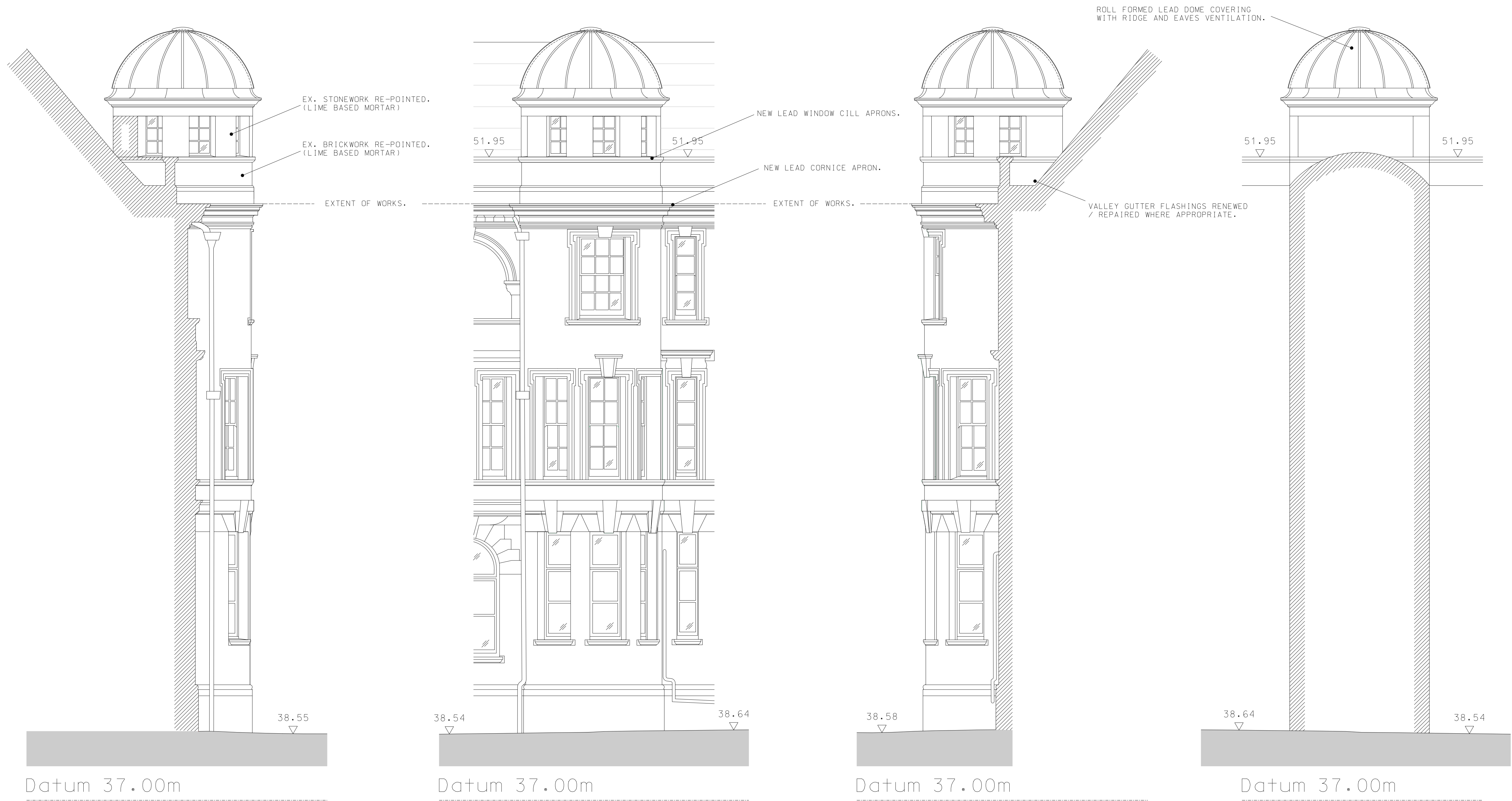
South Turret – Proposed Elevations
