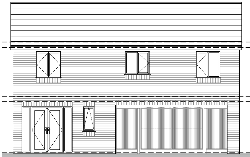
REAR ELEVATION 1:100
