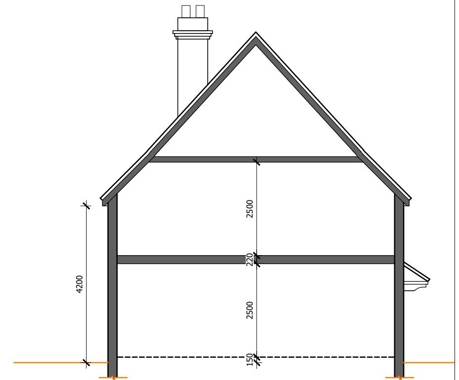
EXISTING SECTION
