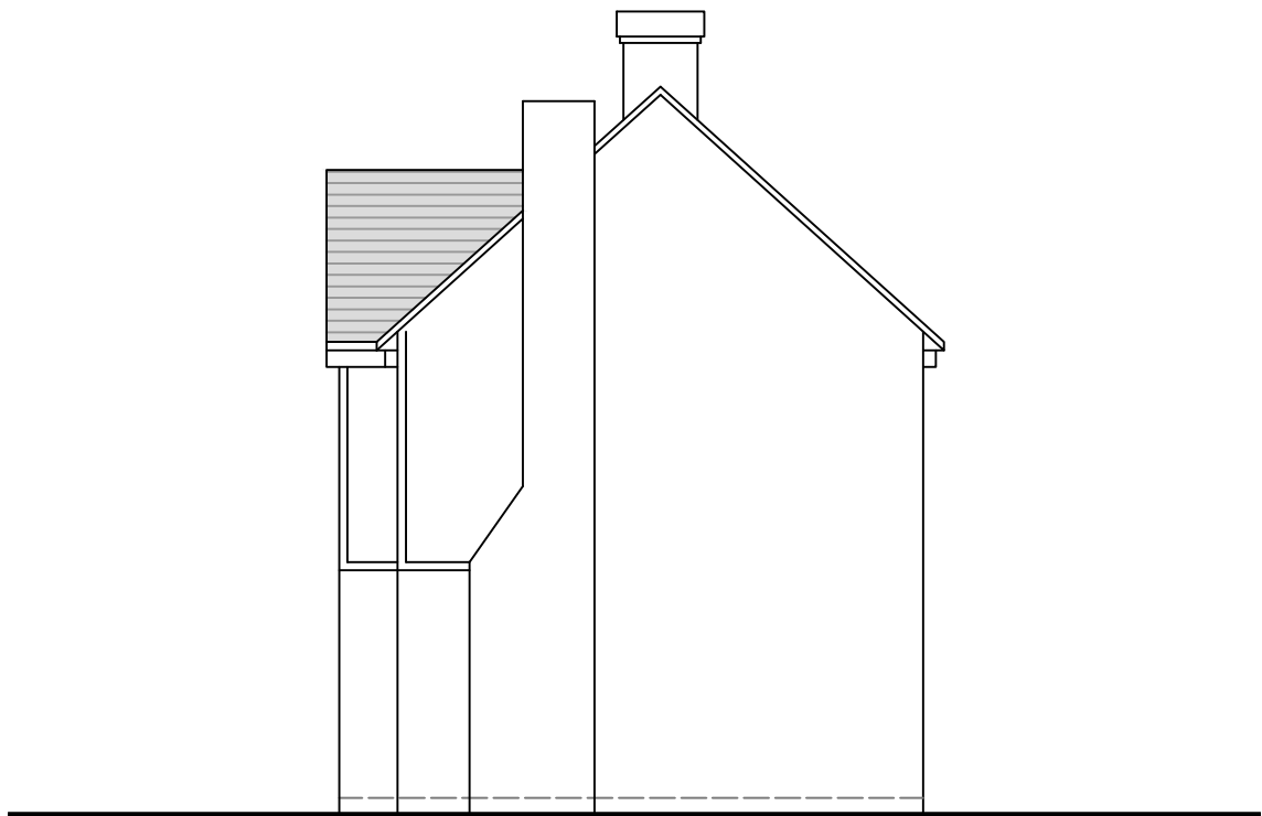
ELEVATION - SIDE 1
