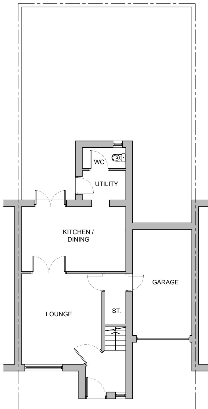
GROUND FLOOR 1:100
