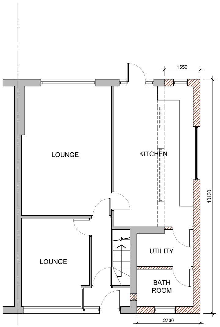
GROUND FLOOR 1:100
