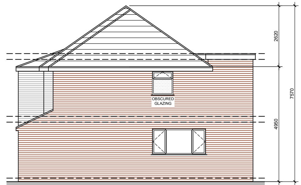
SIDE ELEVATION 1:100
