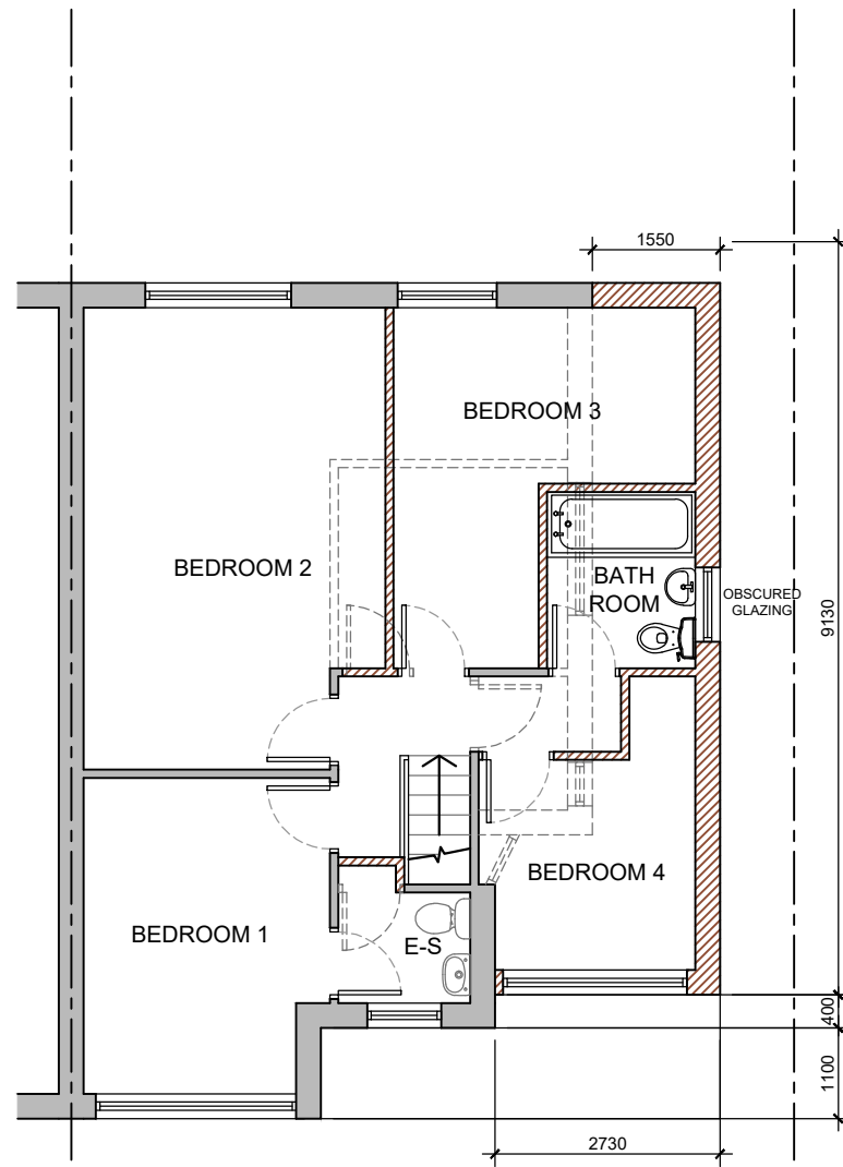
FIRST FLOOR 1:100
