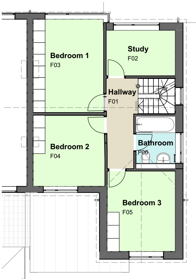
2 01-First Floor 1:100
