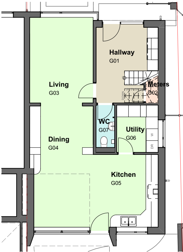
1 GF-Ground Floor 1:100
