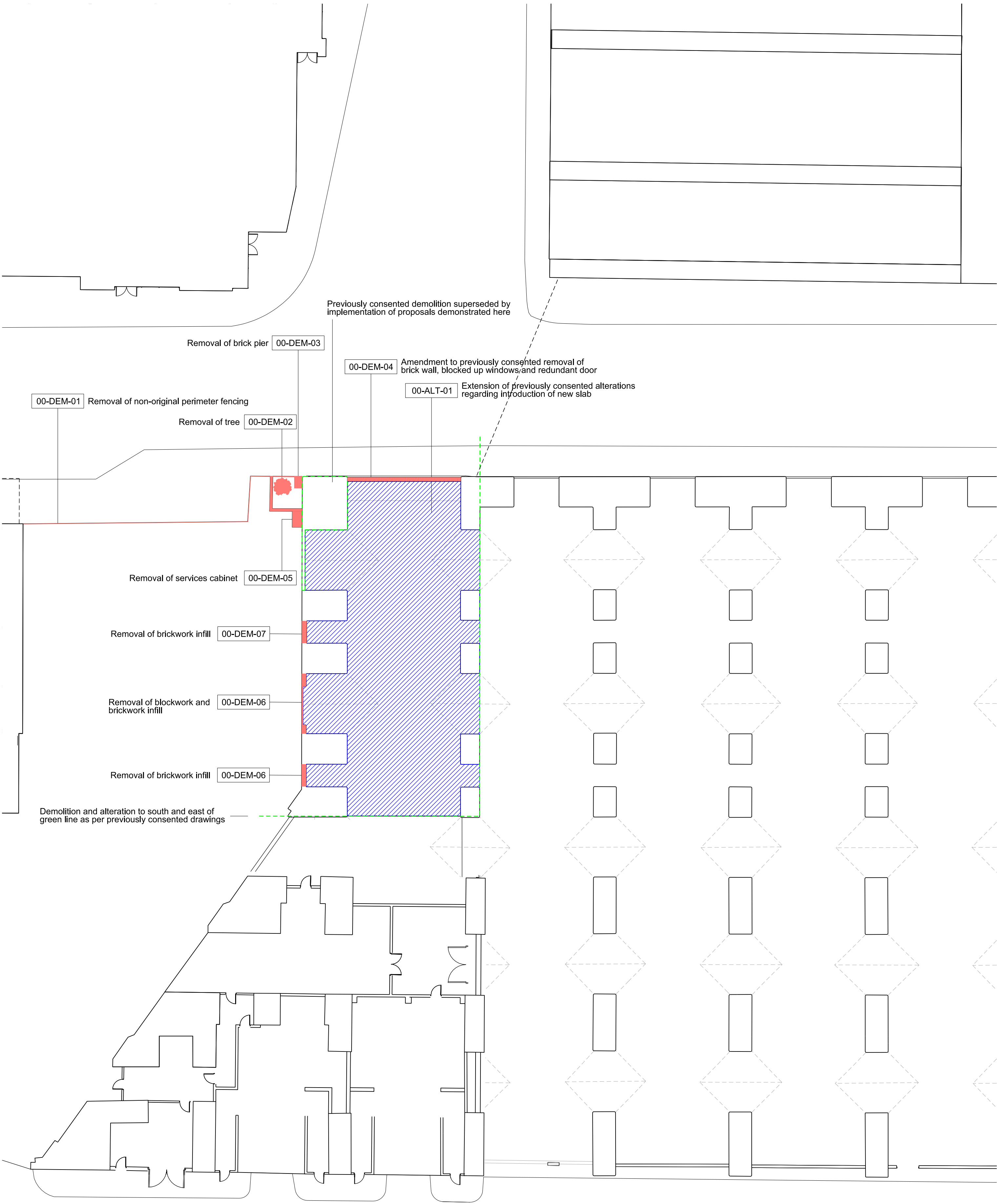
Level 00 Plan
