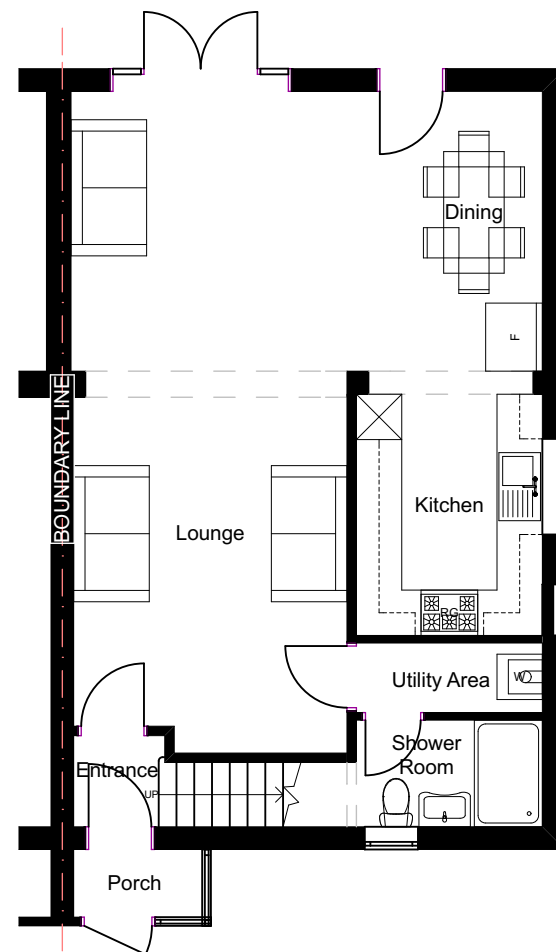
EXISTING GA GROUND FLOOR PLAN
