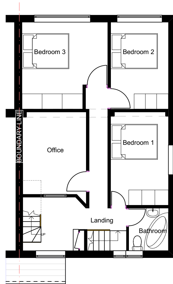
EXISTING GA FIRST FLOOR PLAN
