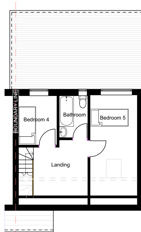
EXISTING GA SECOND FLOOR PLAN
