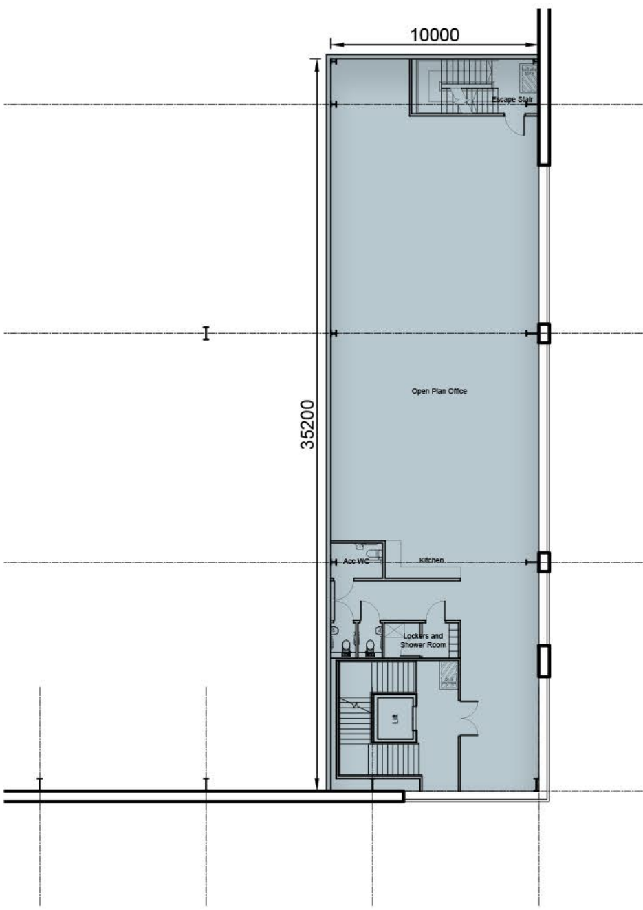
First Floor Office Plan Unit 2a 1:250
