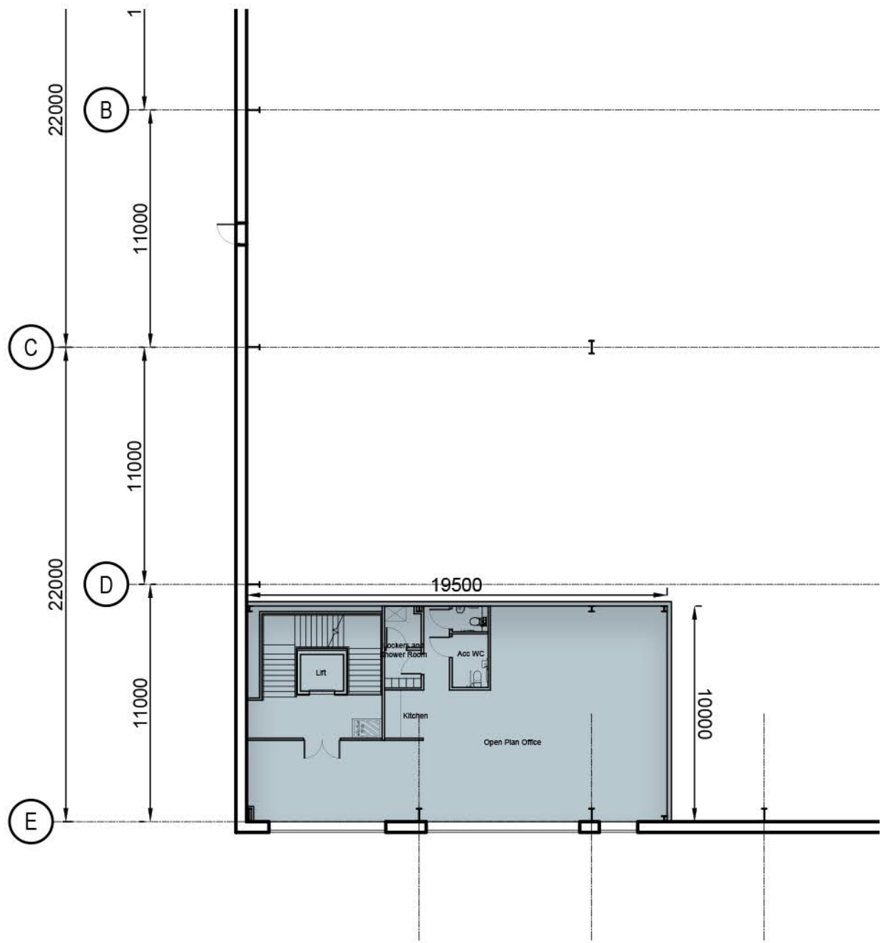
First Floor Office Plan Unit 2d 1:250
