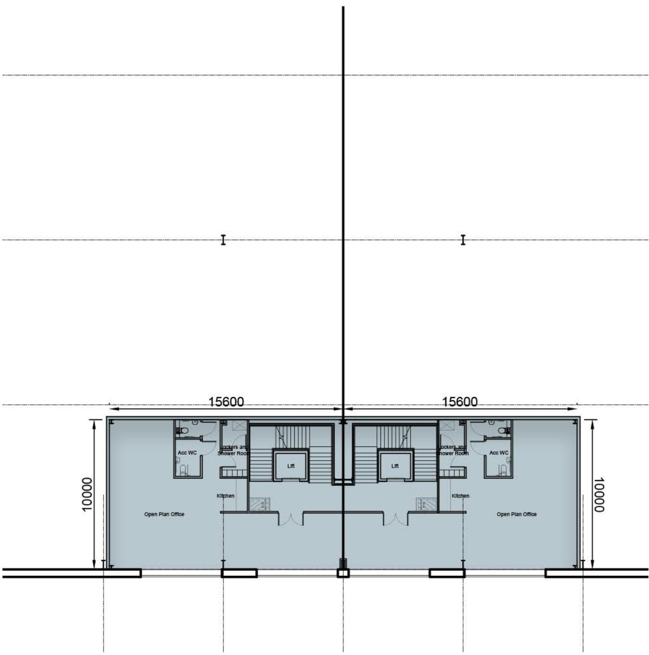
First Floor Office Plan Units 2b and 2c 1:250
