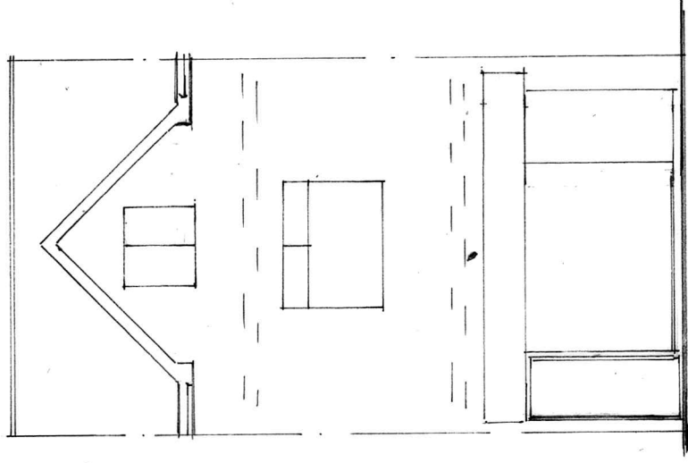
FRONT ELEVATION (PROPOSED)
