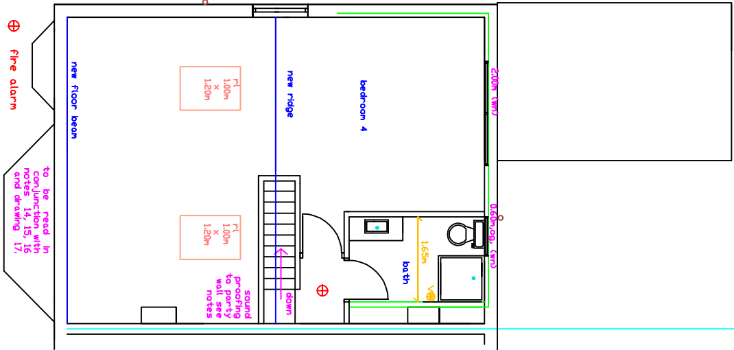
PROPOSED LOFT FLOOR
