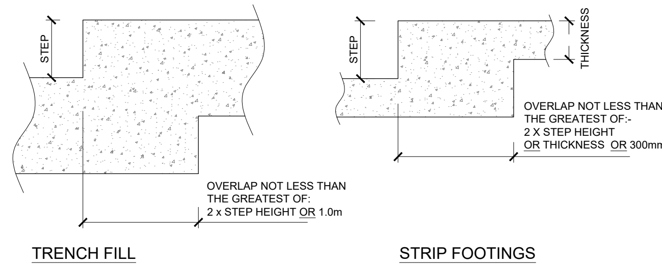
TYPICAL FOUNDATION STEPPING DETAILS (1:20)
