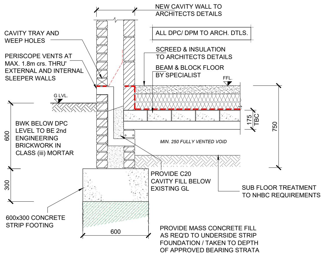
SECTION A - A (1:20)
