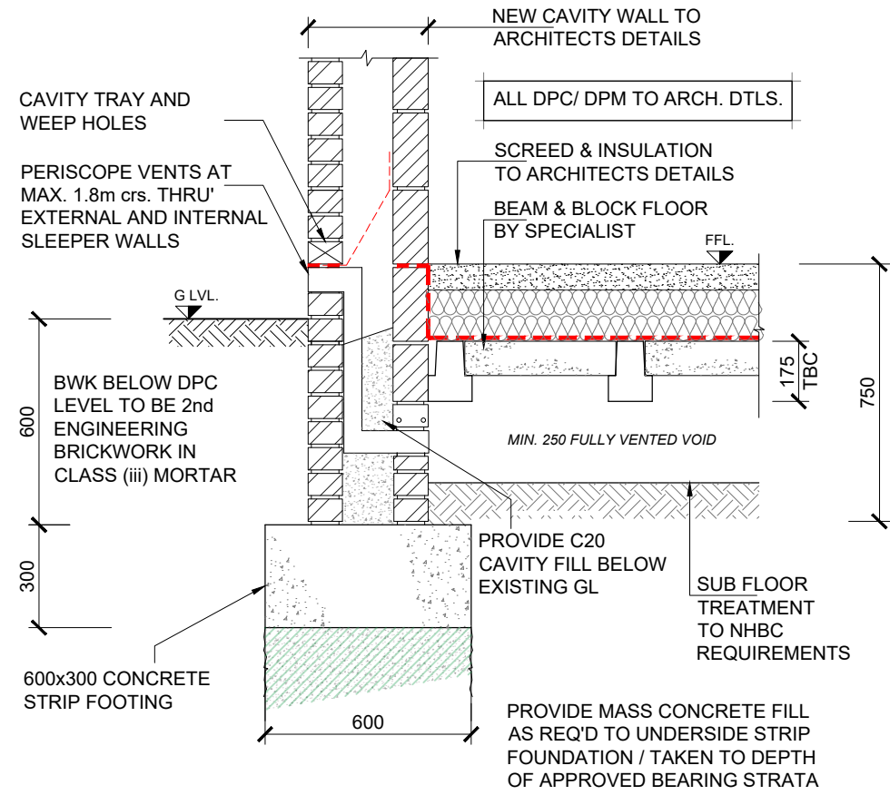
SECTION B - B (1:20)
