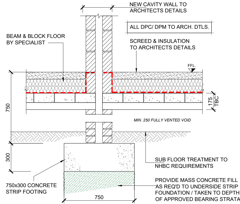
SECTION D - D (1:20)
