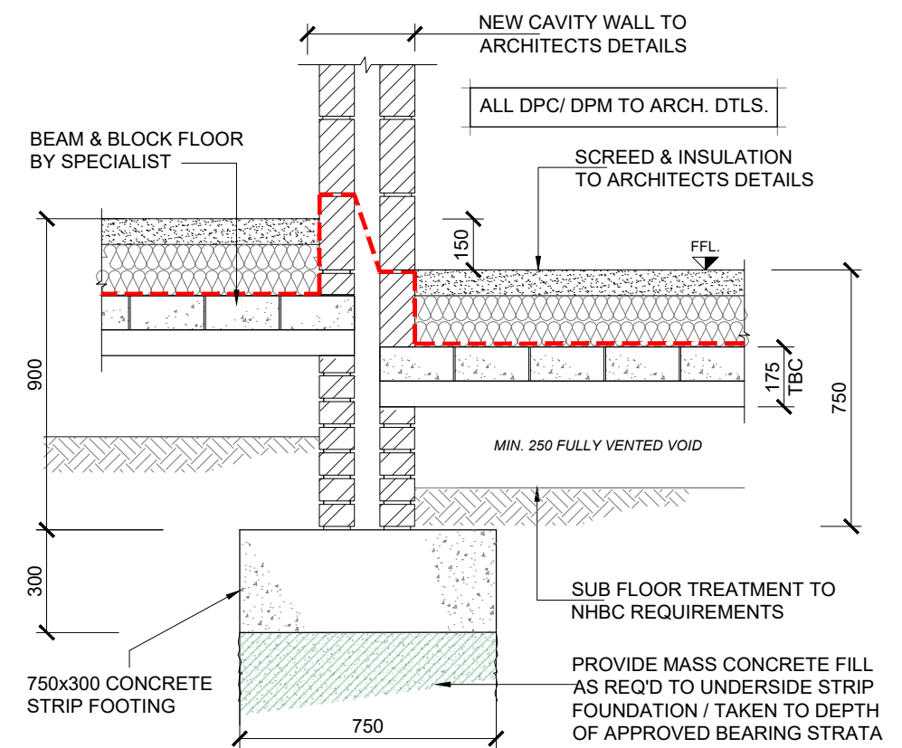
SECTION C - C (1:20)
