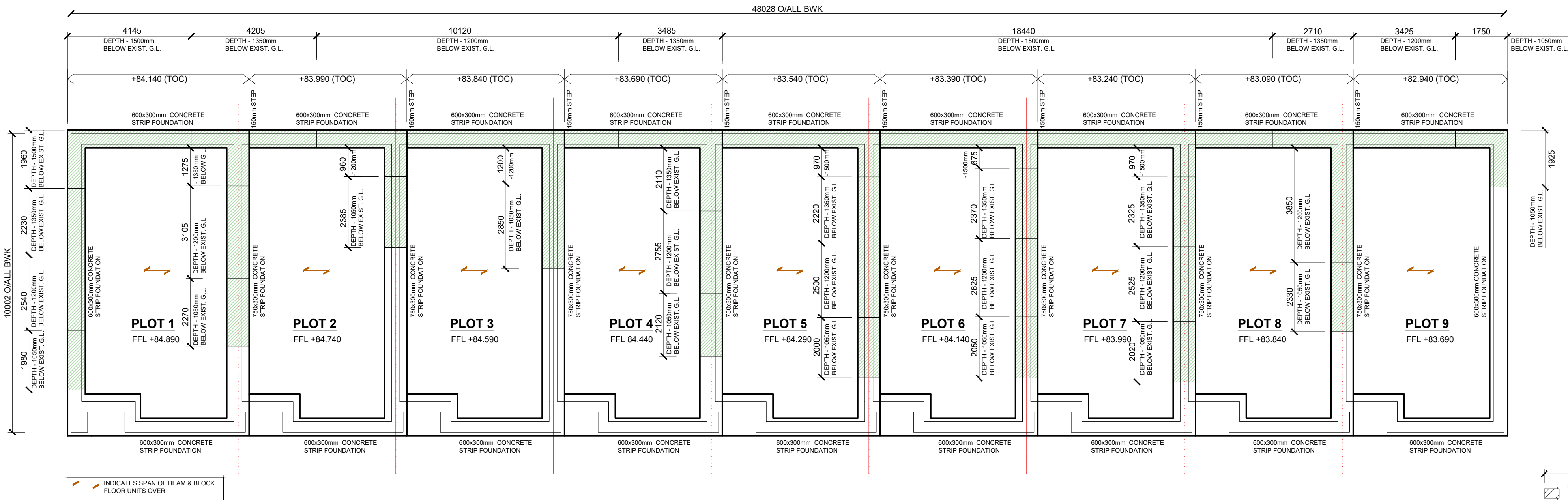
FOUNDATION PLAN (PLOTS 1-9) (1:100)
