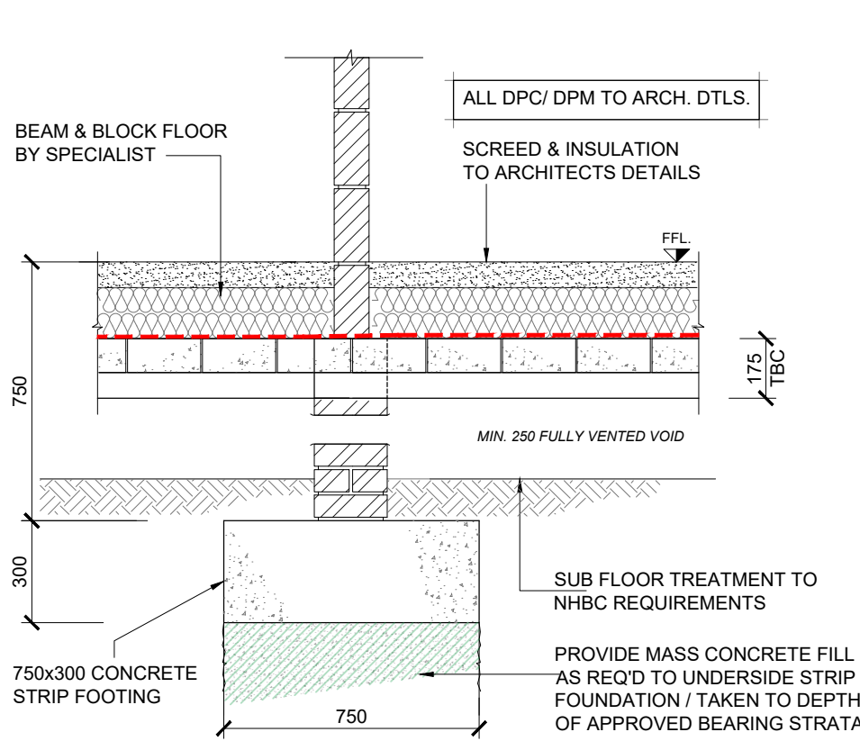
SECTION C - C (1:20)
