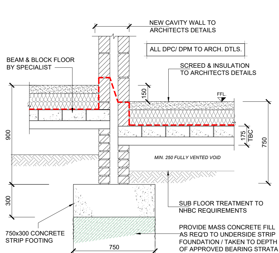
SECTION C - C (1:20)
