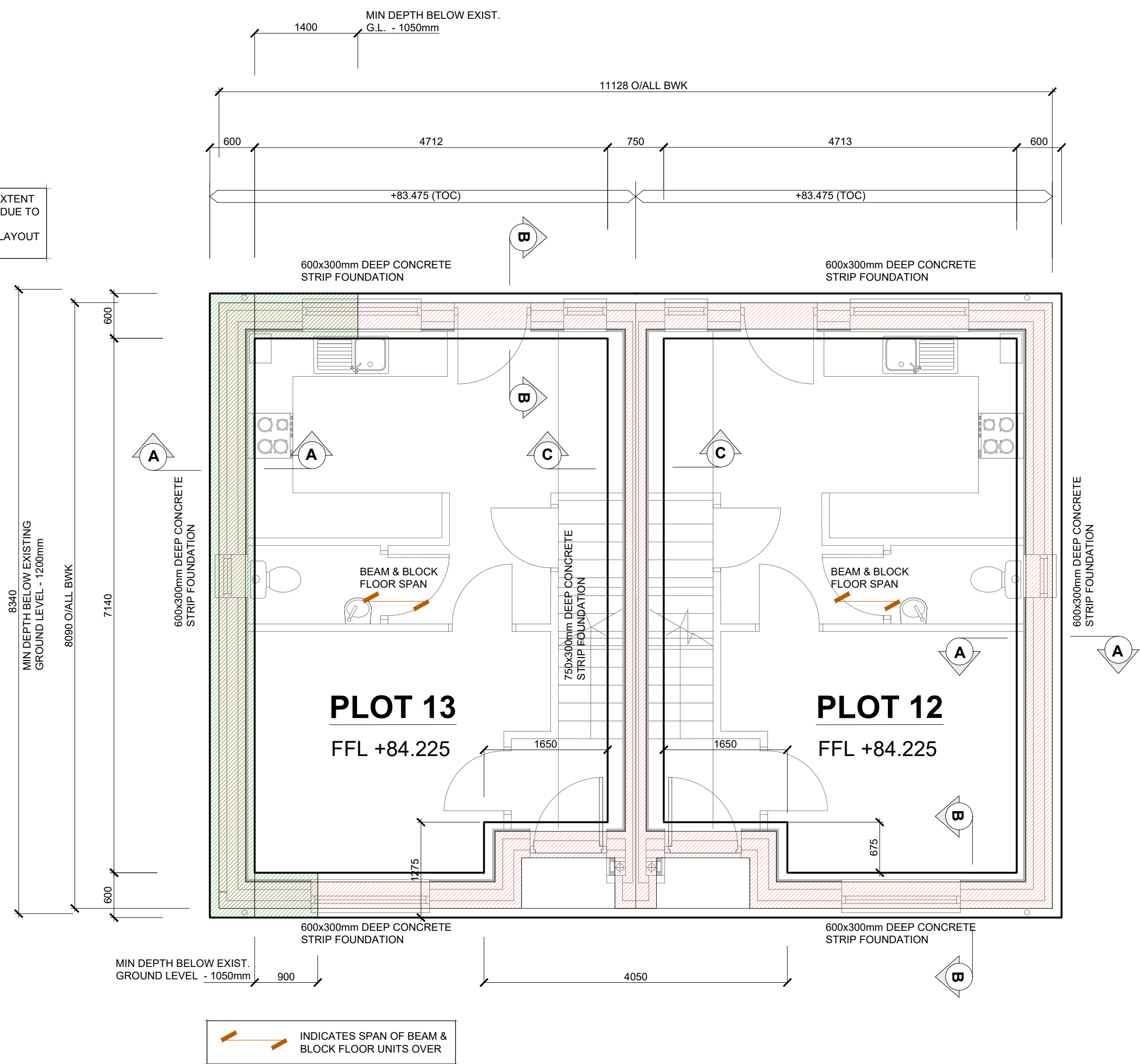
FOUNDATION DETAIL SET-OUT PLAN (1:50)
