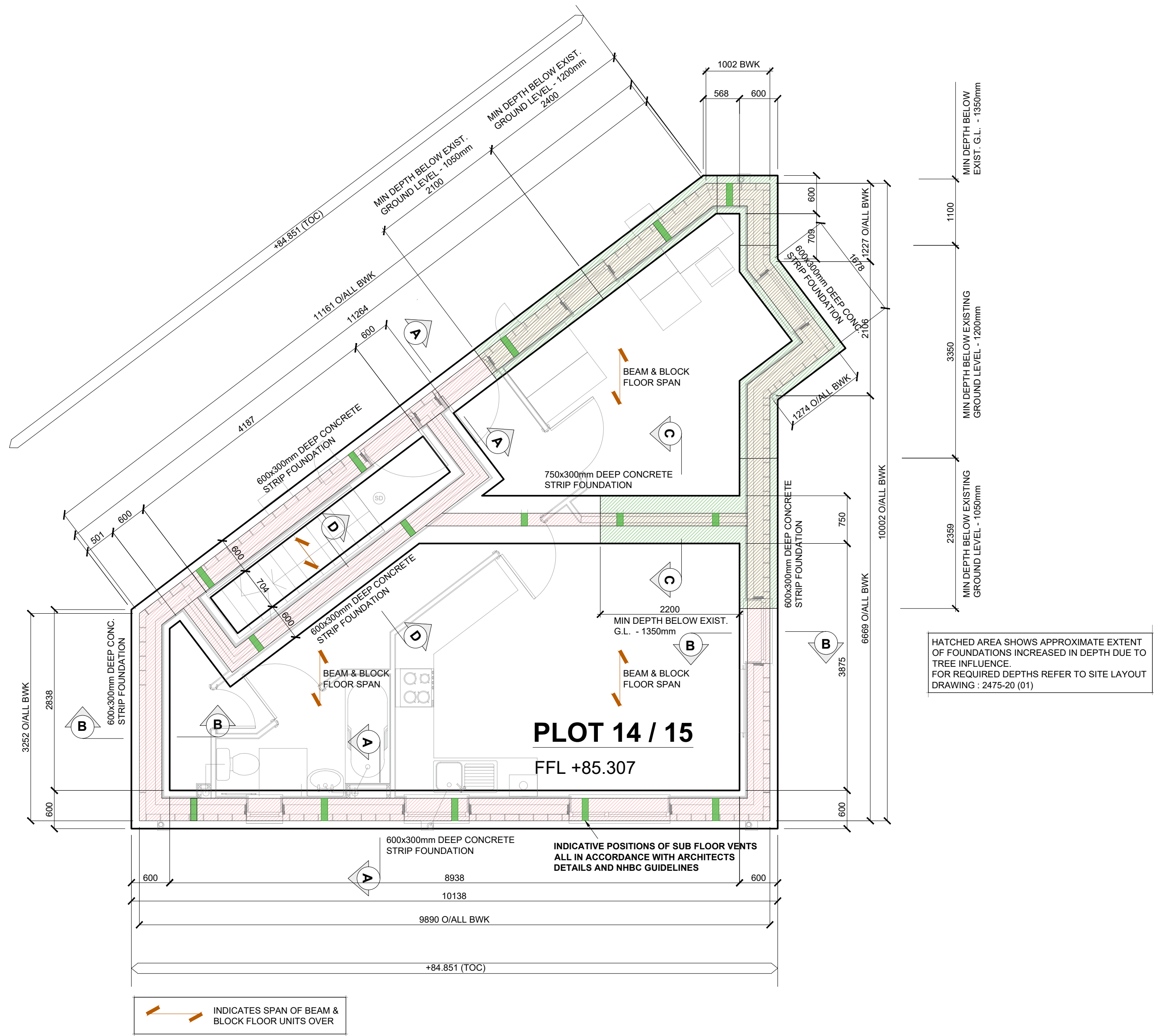
FOUNDATION DETAIL SET-OUT PLAN (1:50)
