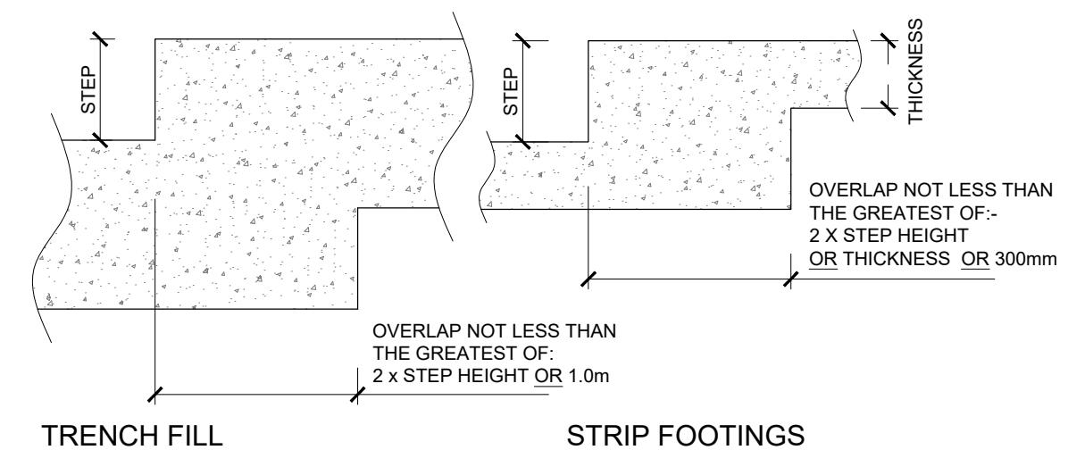
TYPICAL FOUNDATION STEPPING DETAILS (1:20)
