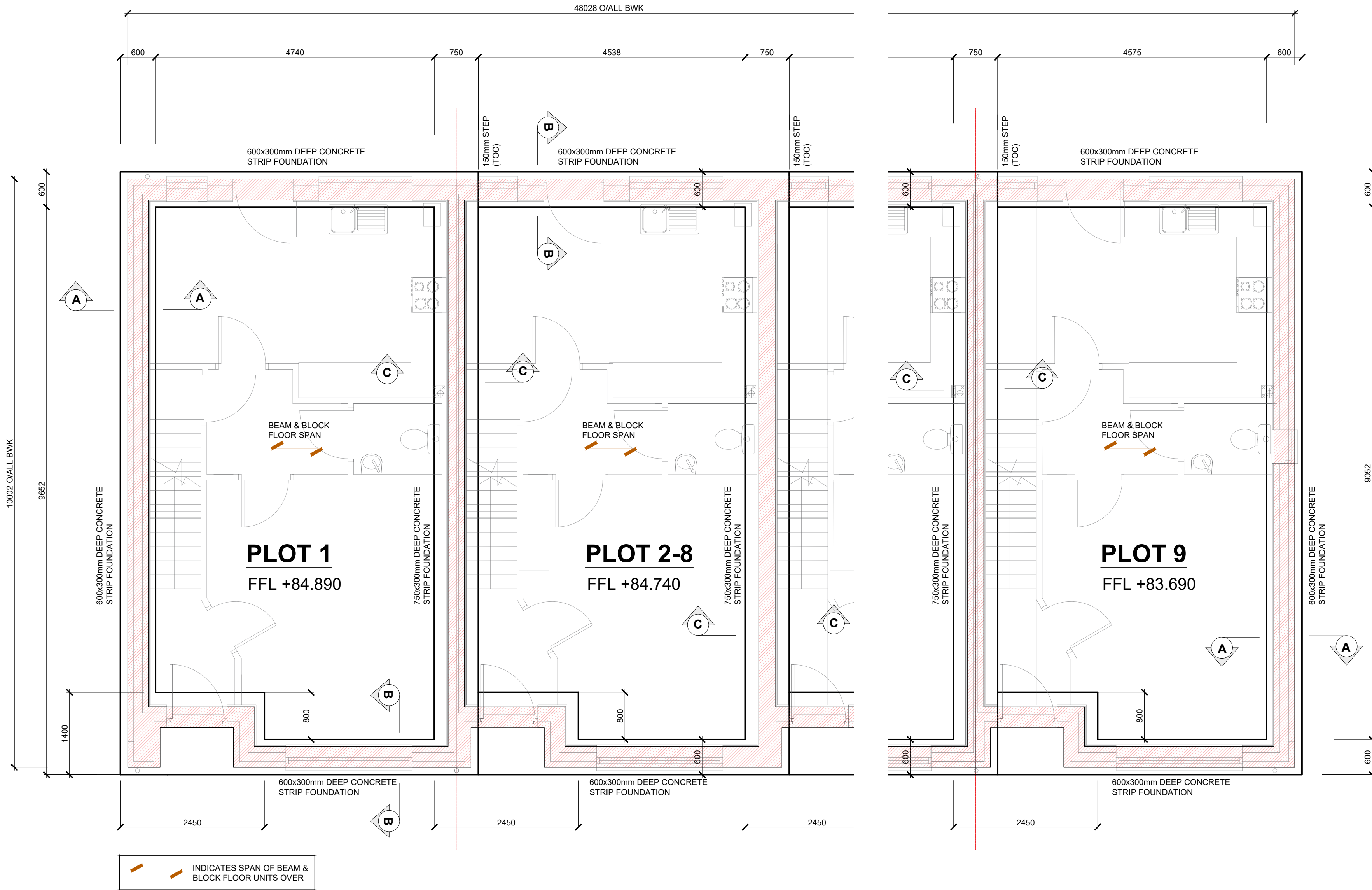
TYPICAL FOUNDATION DETAIL SET-OUT PLAN (1:50)
