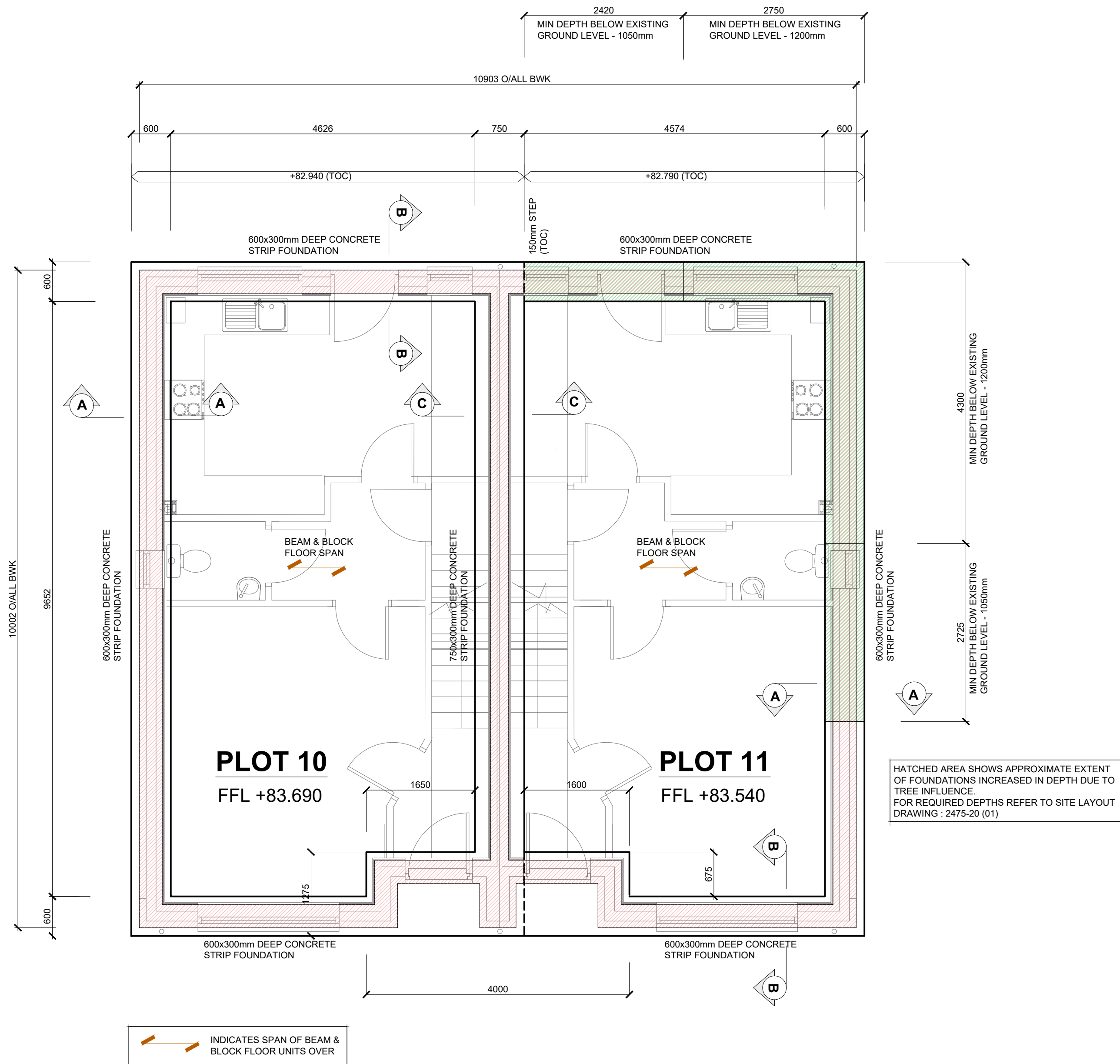
FOUNDATION DETAIL SET-OUT PLAN (1:50)
