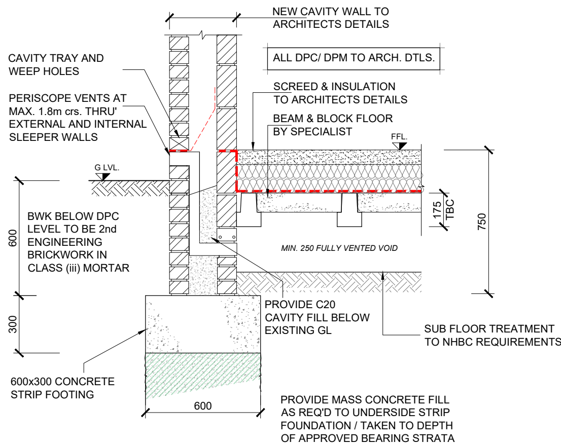
SECTION B - B (1:20)
