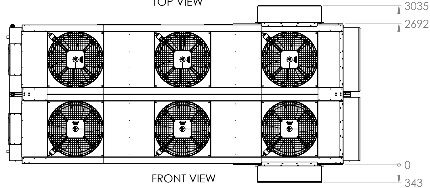
TOP VIEW
