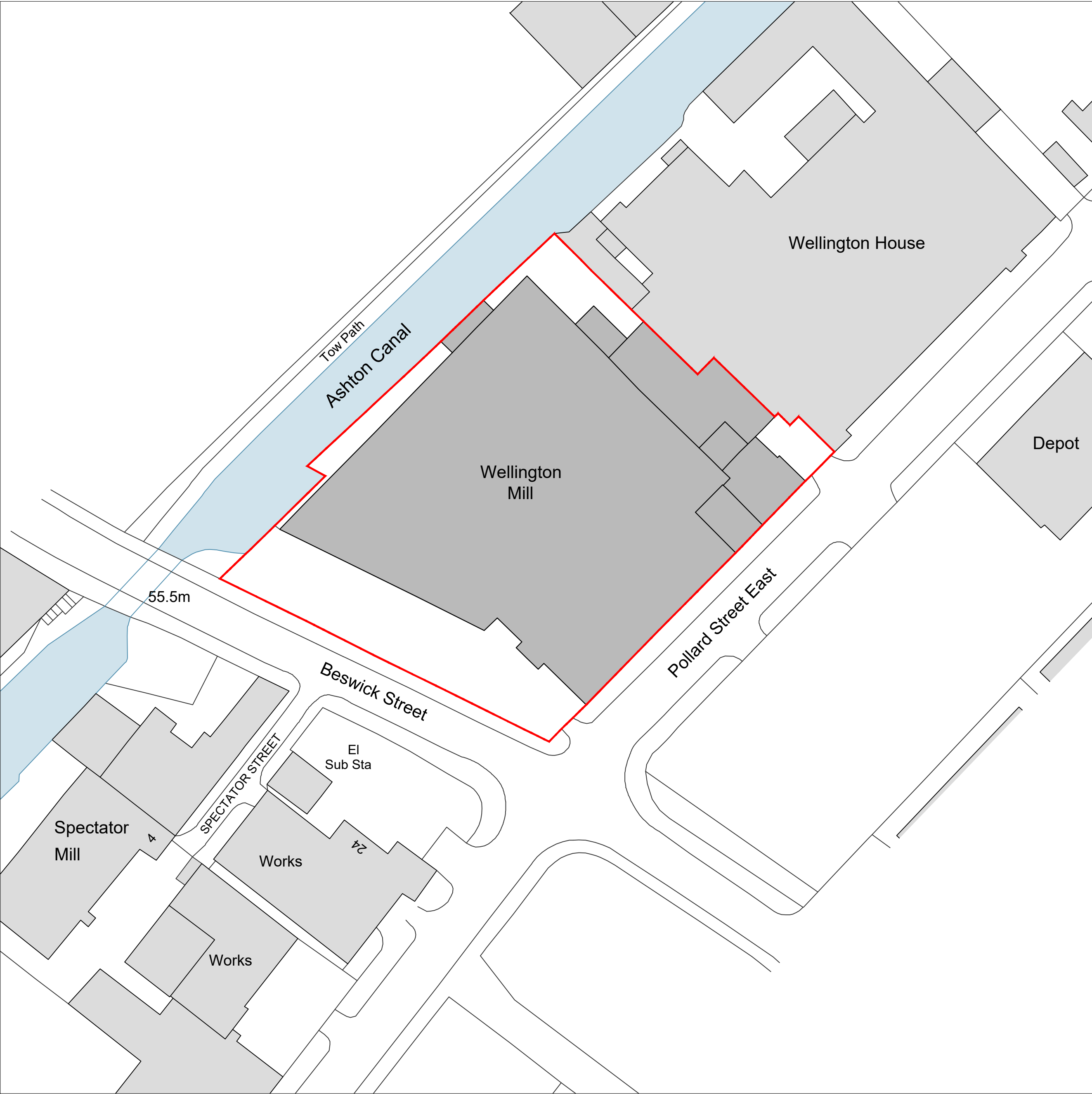
Site Location Plan Scale 1:500 Scale Bar 1:500 @ A1
