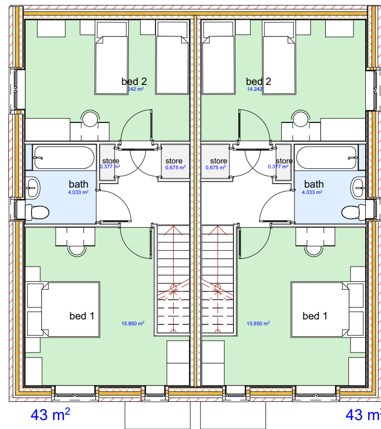
2 01-First Floor 1:100
