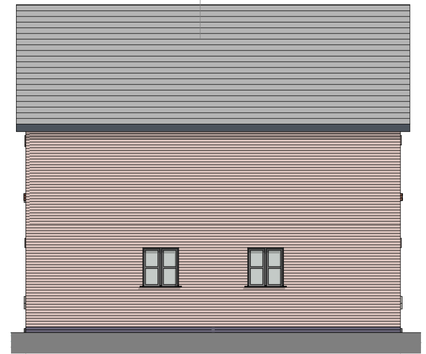
Rear Elevation 1:100
