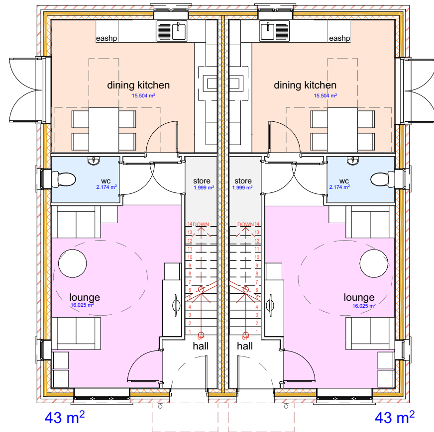
1 GF-Ground Floor 1:100
