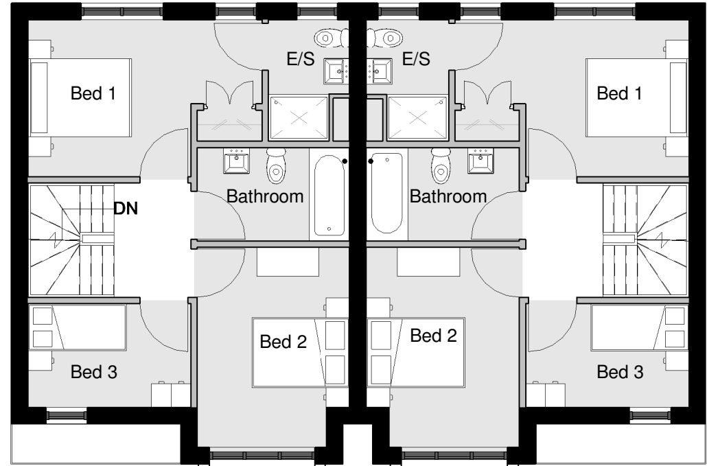
1 Proposed First Floor 1 : 100
