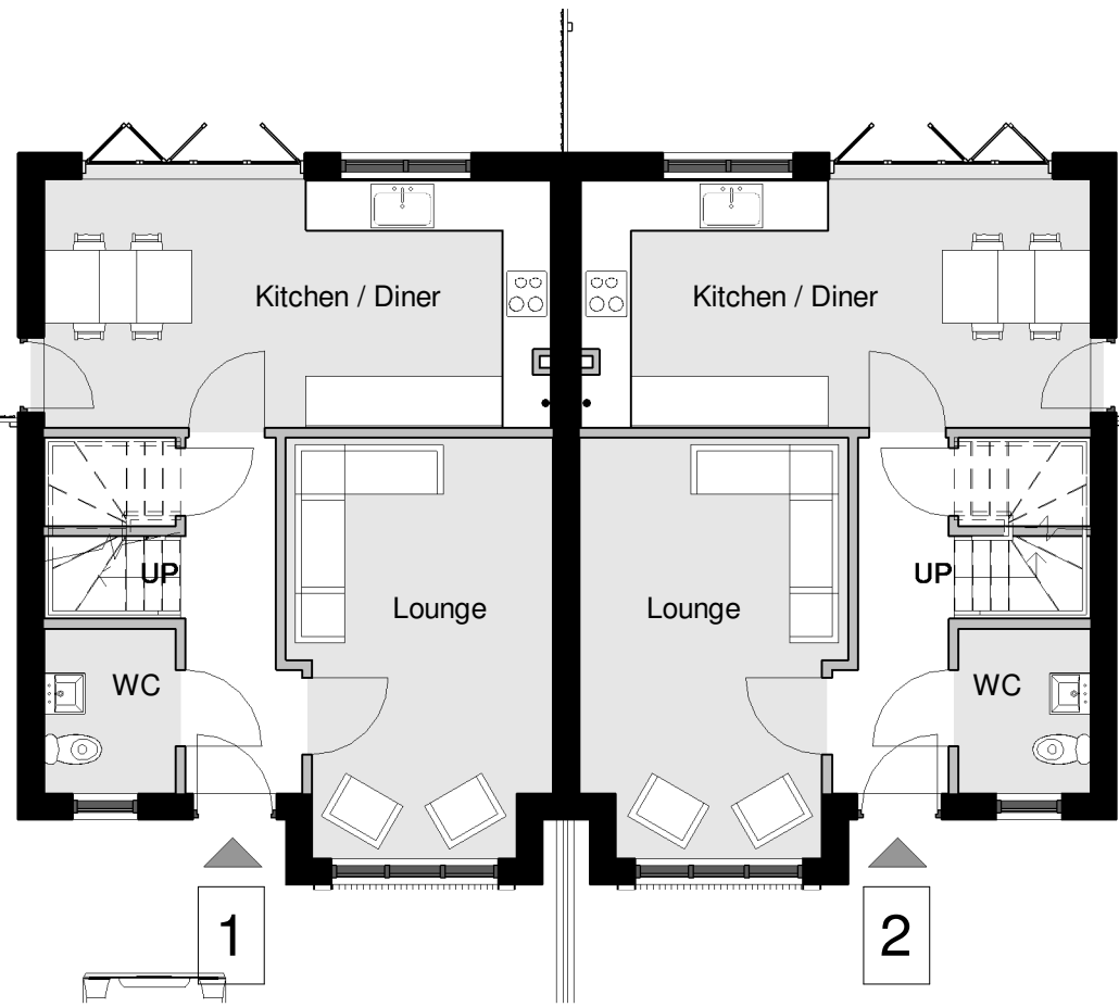
G Proposed Ground Floor 1 : 100
