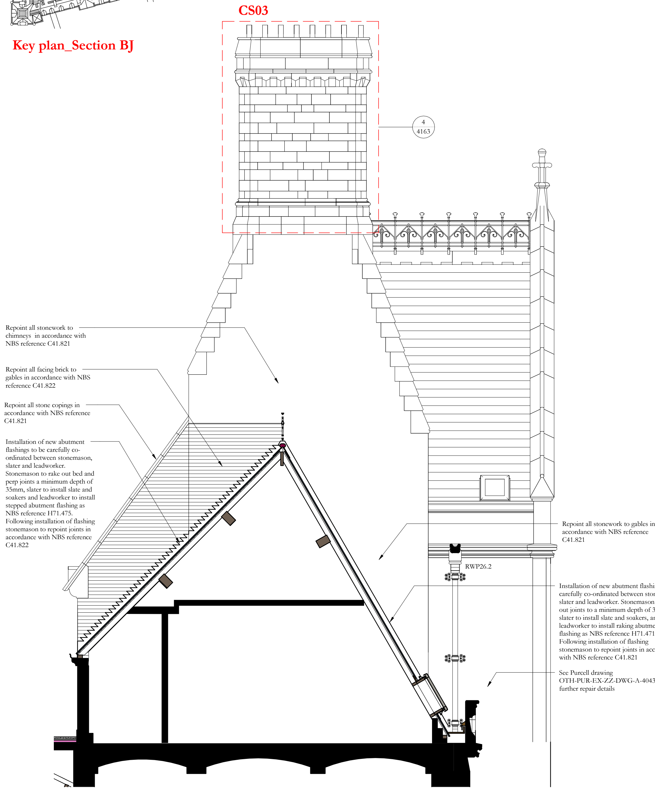
Section BJ
