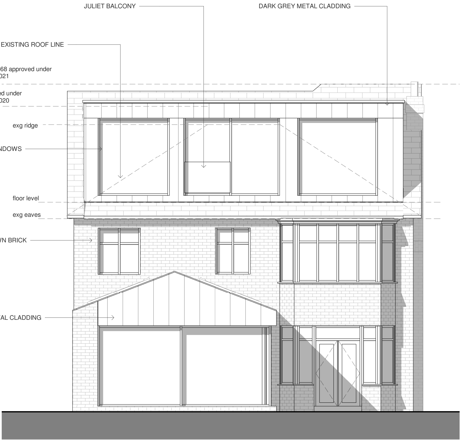
PROPOSED ELEVATIONS - North-West 1 : 50
