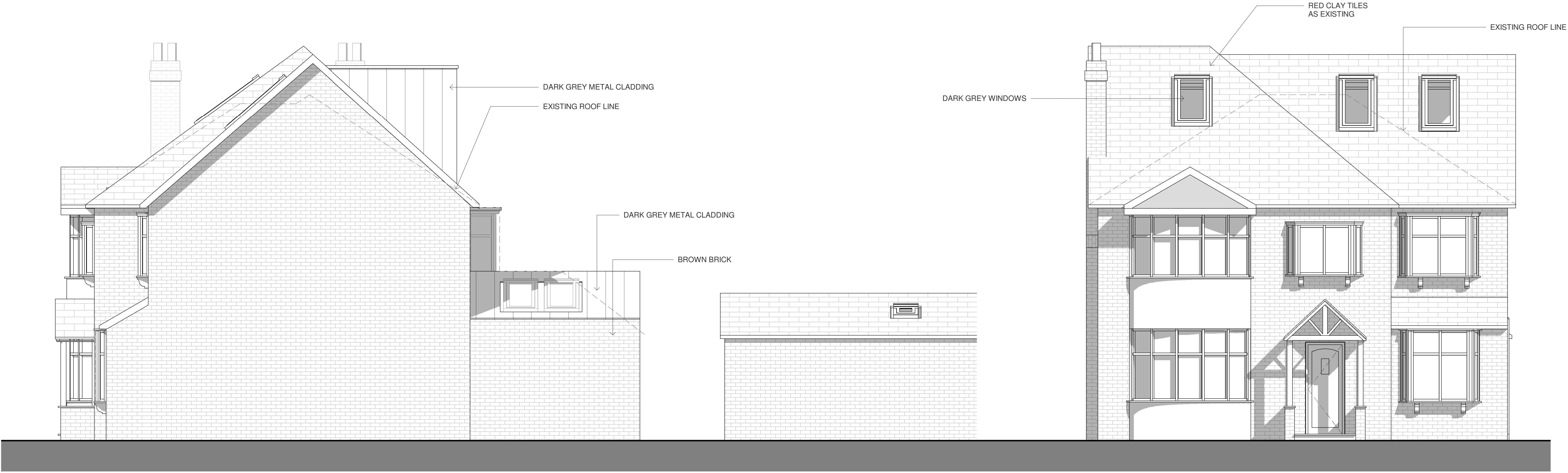
PROPOSED ELEVATIONS - North-East 1 : 50
