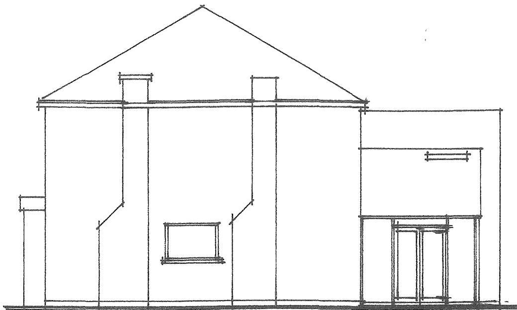
S/ WEST ELEVATION
