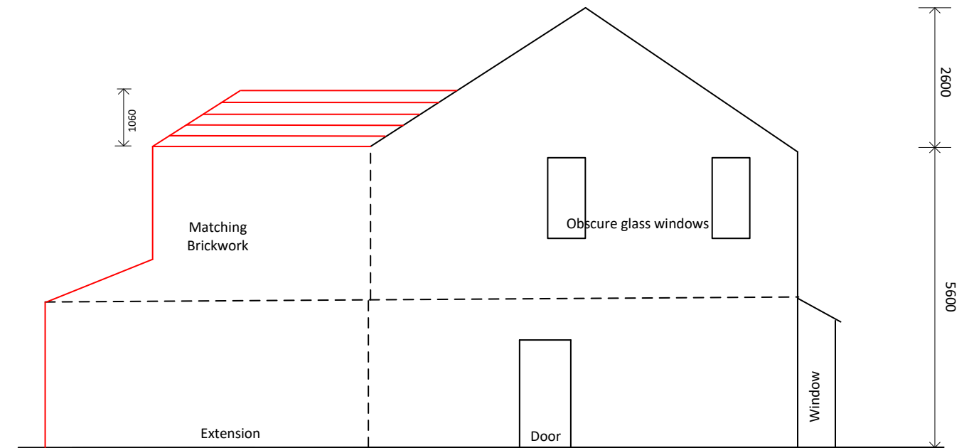
PROPOSED SIDE ELEVATION (from H. No. 76)
