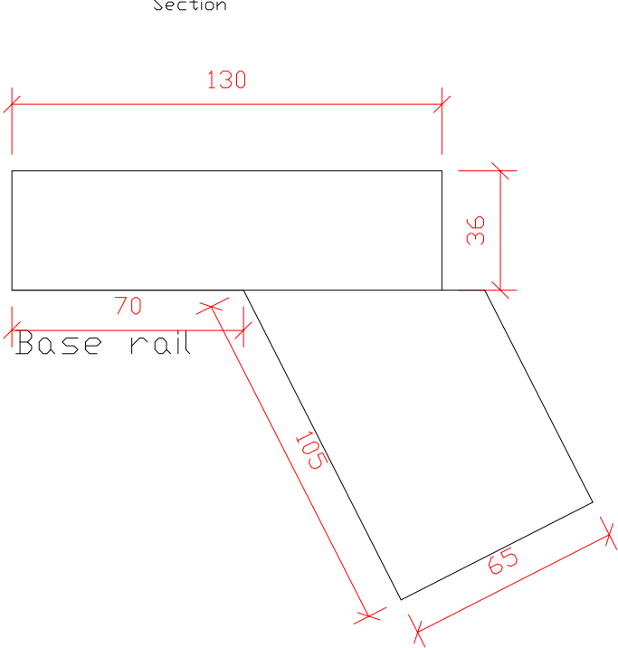
Section
