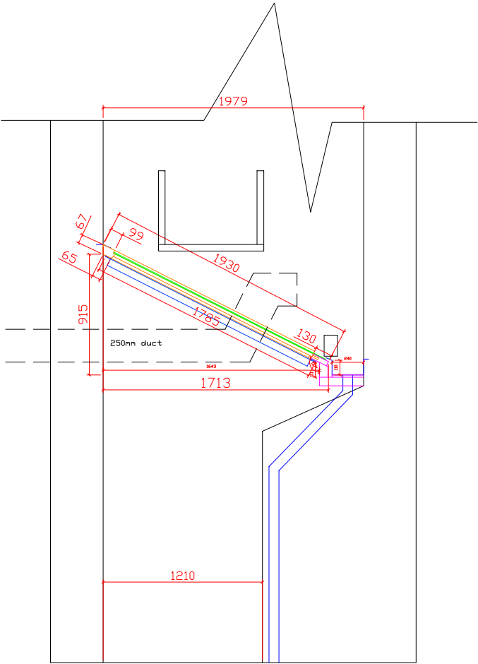
Section
