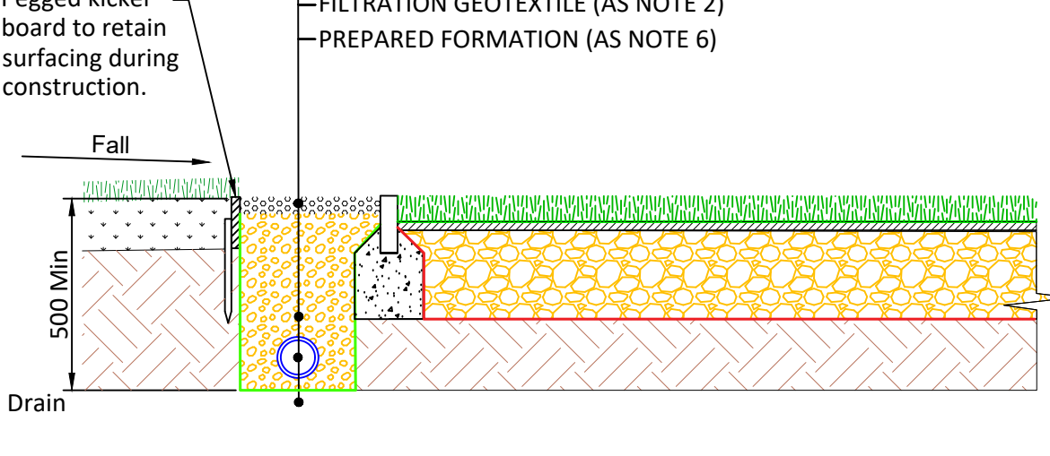
SECTION C-C THROUGH PERIMETER FILTER-RAIN WITH CONVEYANCE PIPE
