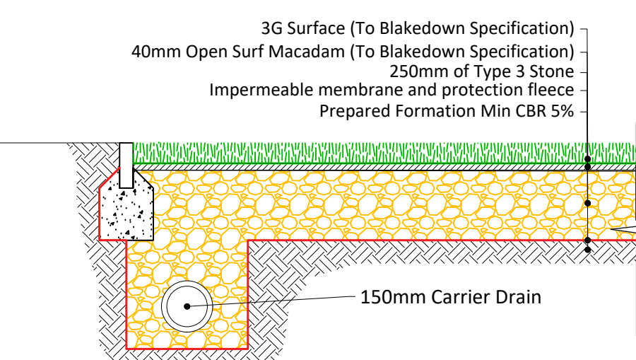
SECTION A-A 150mm CARRIER DRAIN DETAIL
