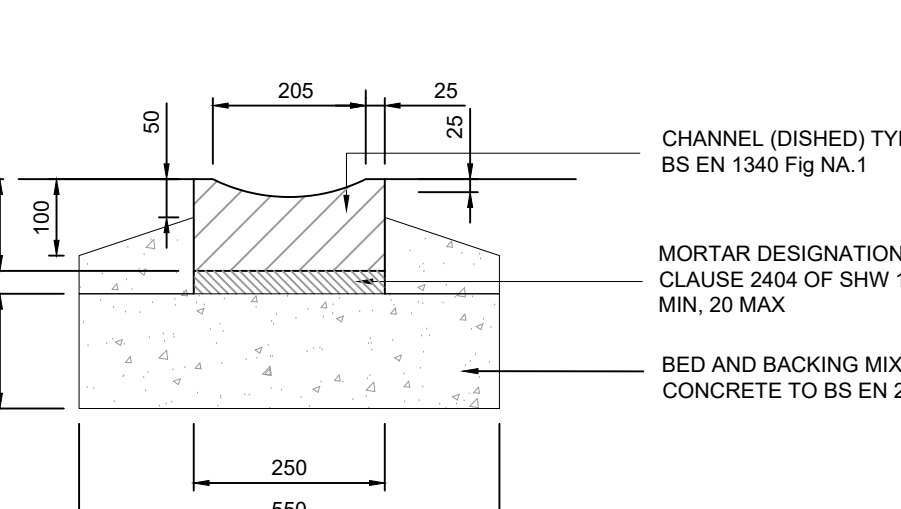
DISHED CHANNEL TYPE CD
