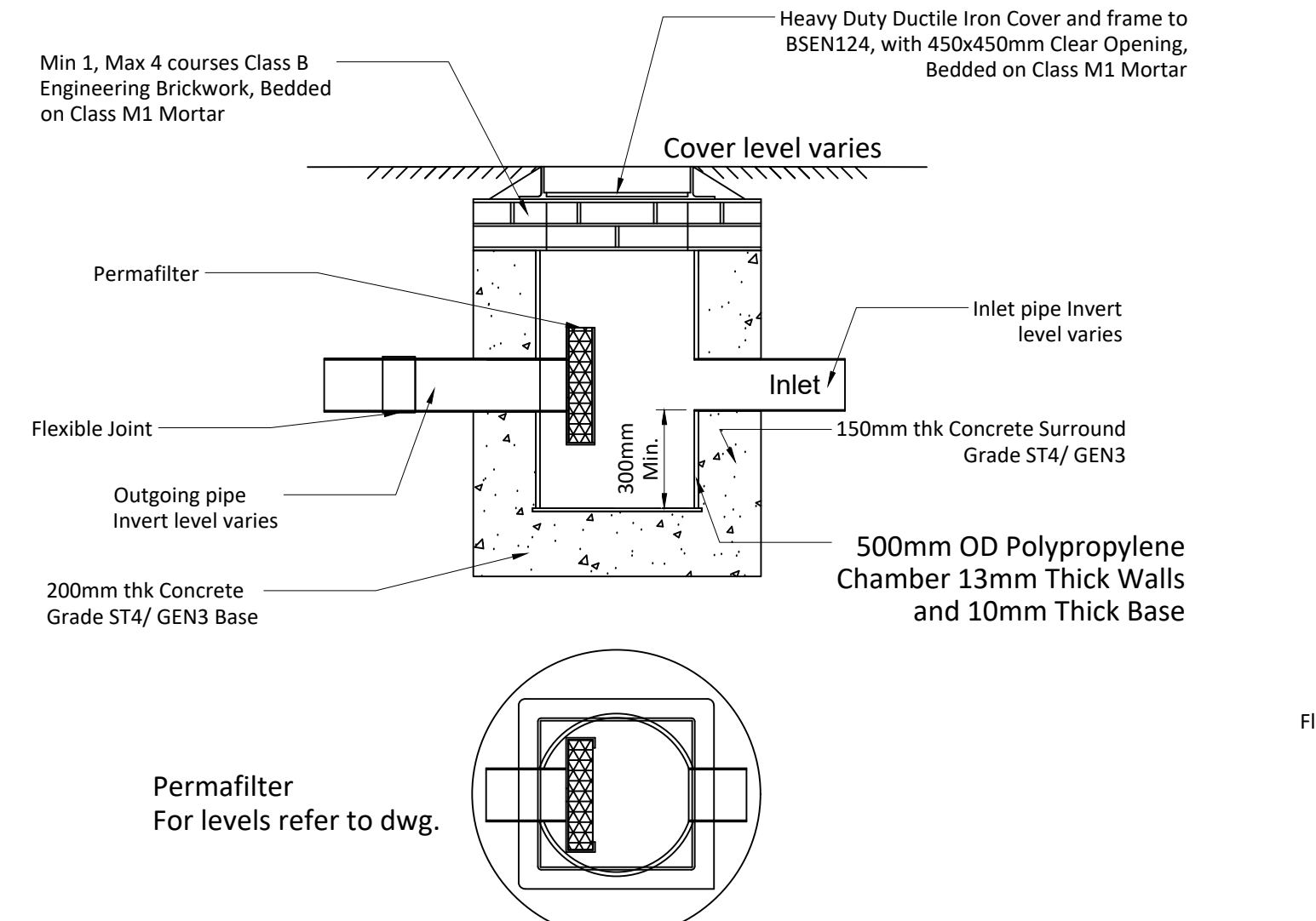
7500 CATCHPIT INSPECTION CHAMBER INCORPORATING DEBRIS DEVICE
