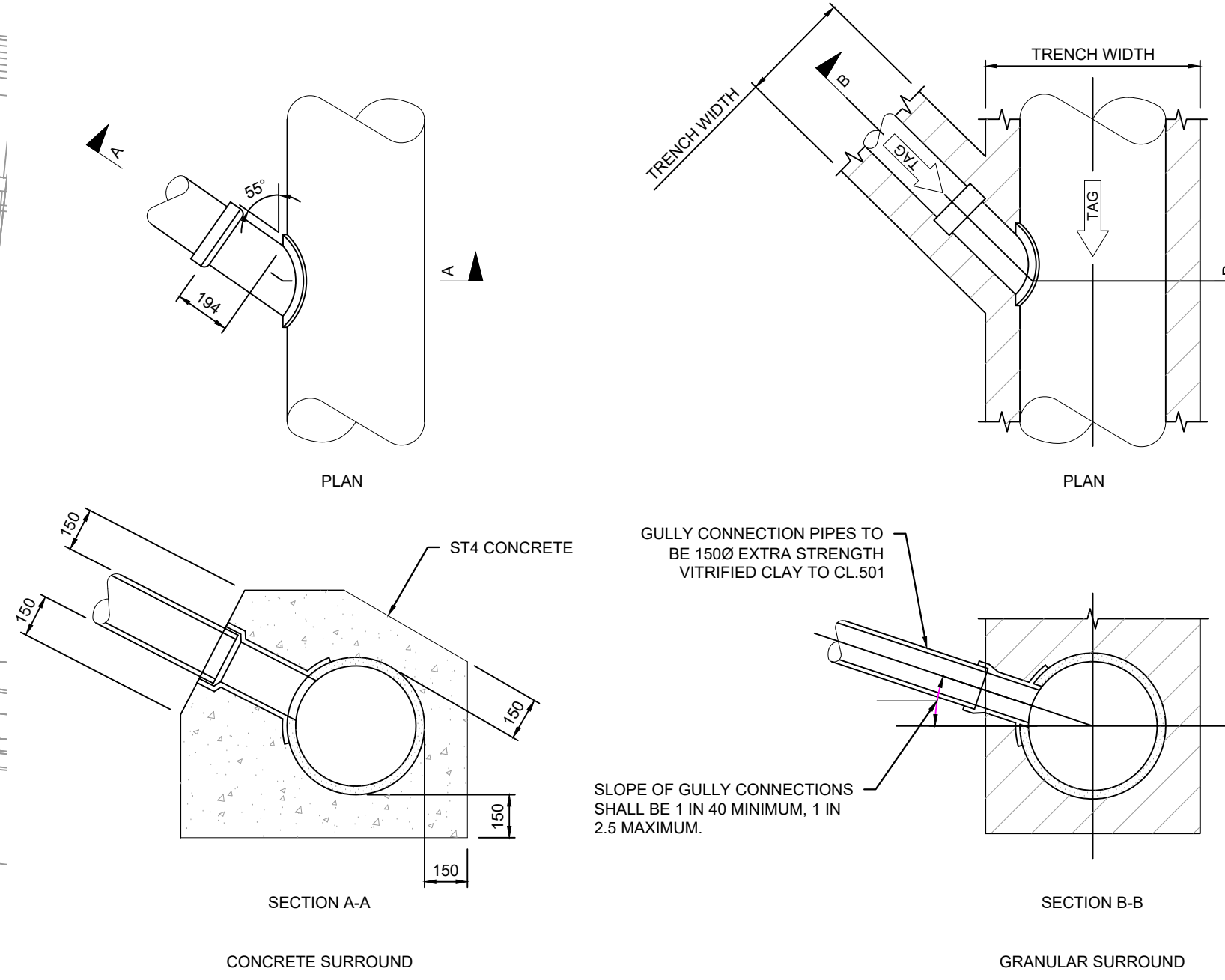
SADDLE CONNECTION DETAILS
