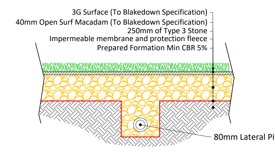
SECTION B-B 80mm LATERAL DRAIN DETAIL
