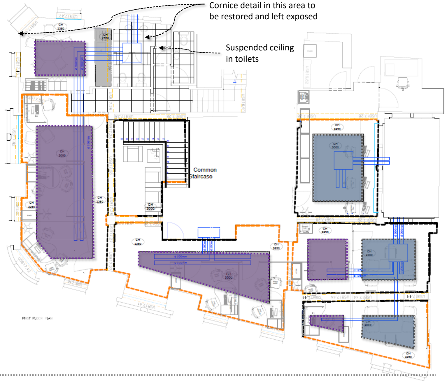
IMAGE SHOWING EXISTING CEILING MADE OF PLASTERBOARD RAFTS
