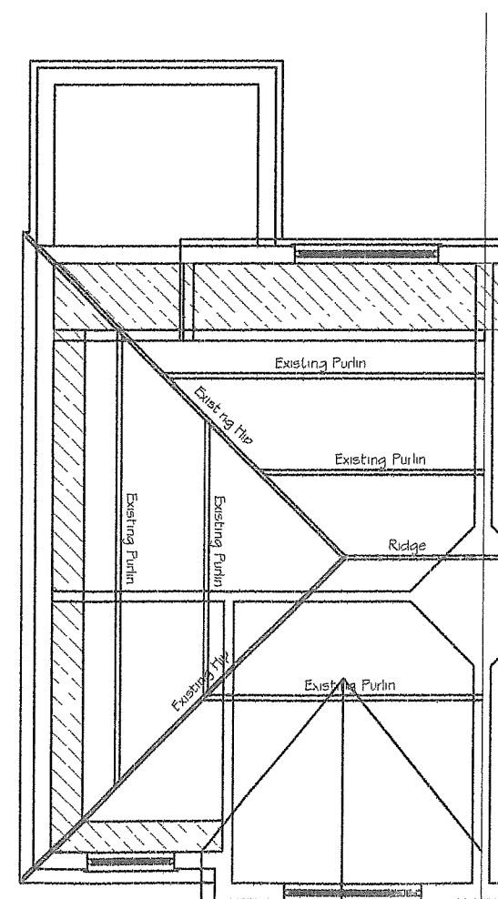
Existing Loft Floor Plan
