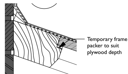
7 Head Detail - Plywood Infill Scale: 1:5
