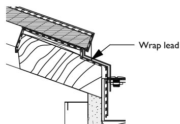
8 Base Detail - Plywood Infill Scale: 1:5
