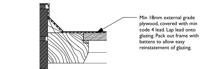
5 Jamb Detail - Plywood Infill Scale: 1:5
