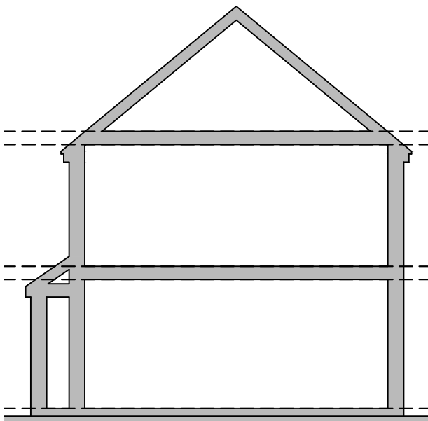
SIDE ELEVATION 1:100
