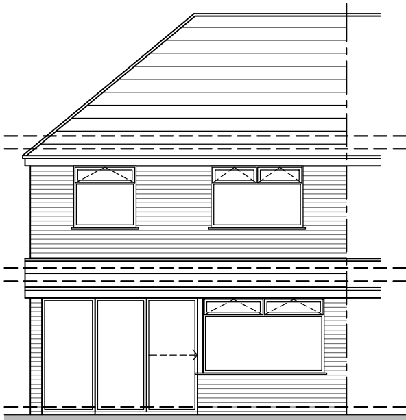
FRONT ELEVATION 1:100
