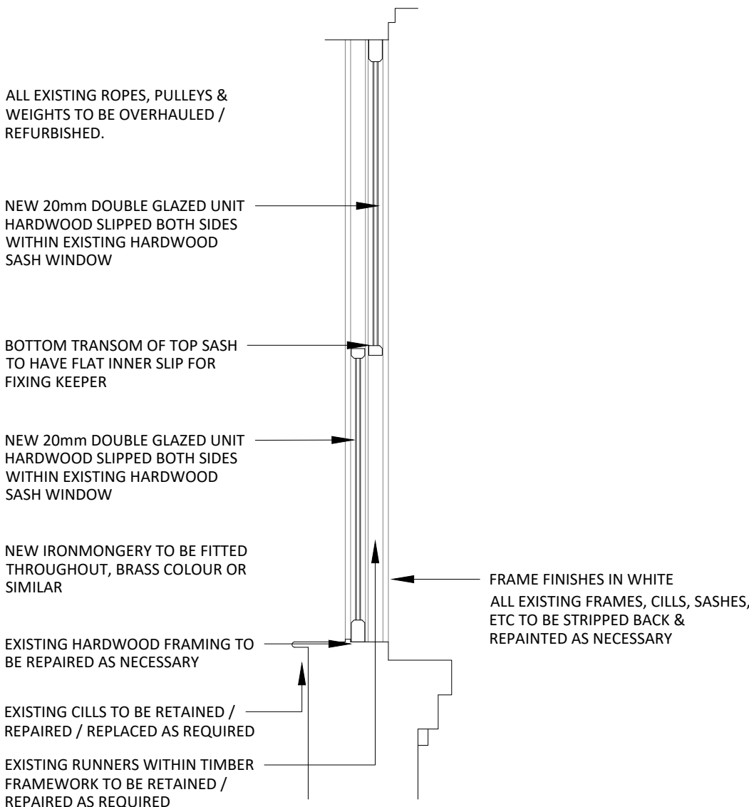
02 1ST FLOOR SASH WINDOW - TYPE A 500 SECTION
