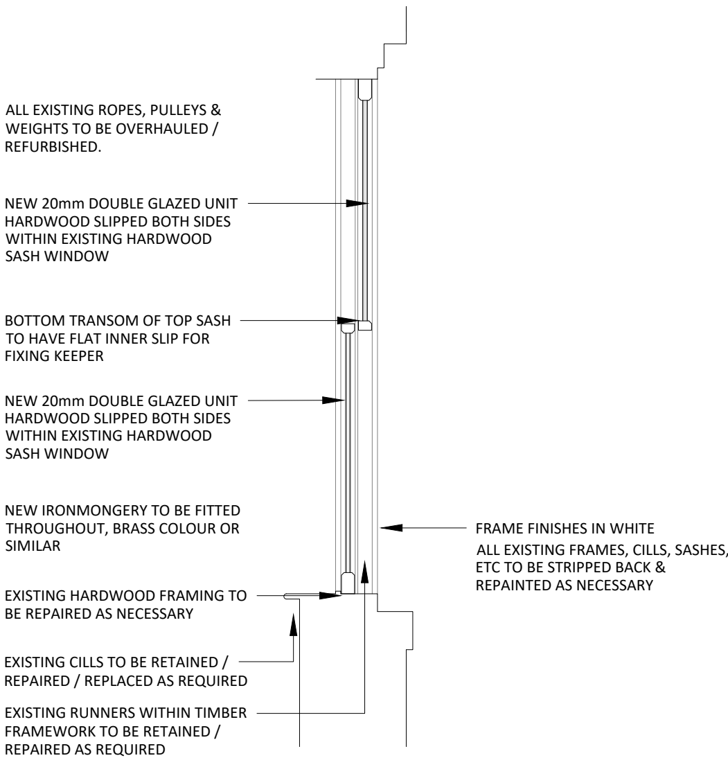
04 2ND FLOOR SASH WINDOW - TYPE B 500 SECTION
