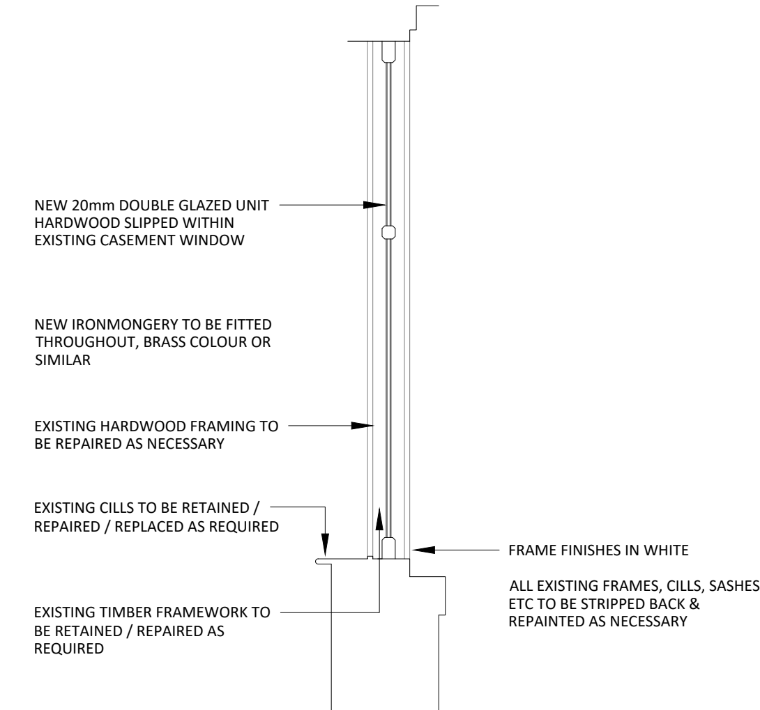
10 CURVED WINDOW PROFILE 500 SECTION
