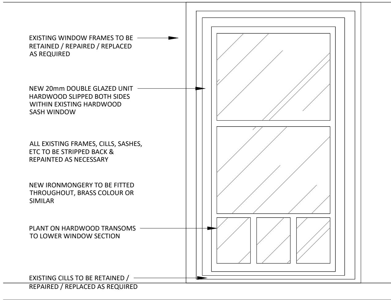
05 3RD FLOOR SASH WINDOW - TYPE C 500 ELEVATION
