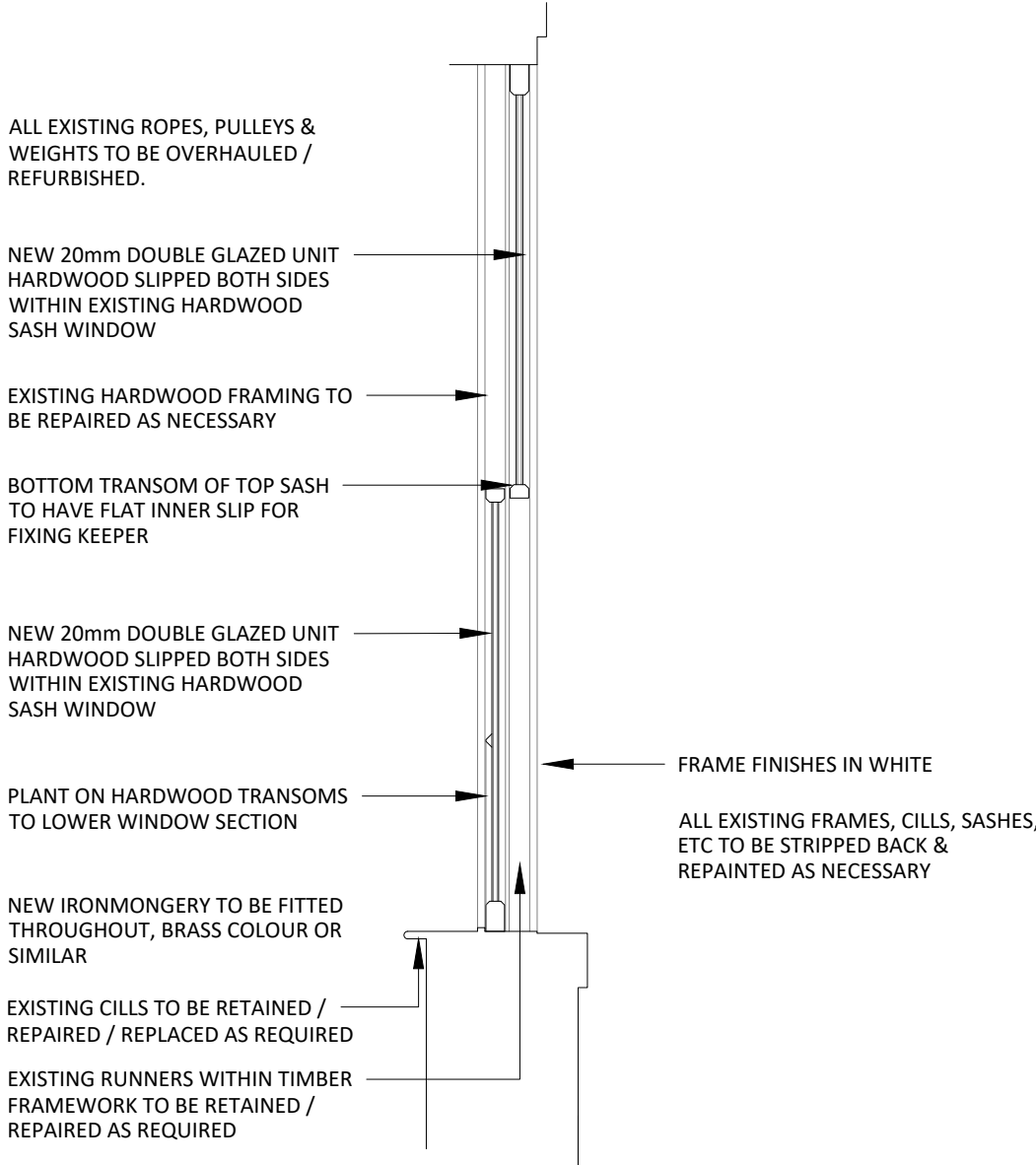
06 3RD FLOOR SASH WINDOW - TYPE C 500 SECTION
