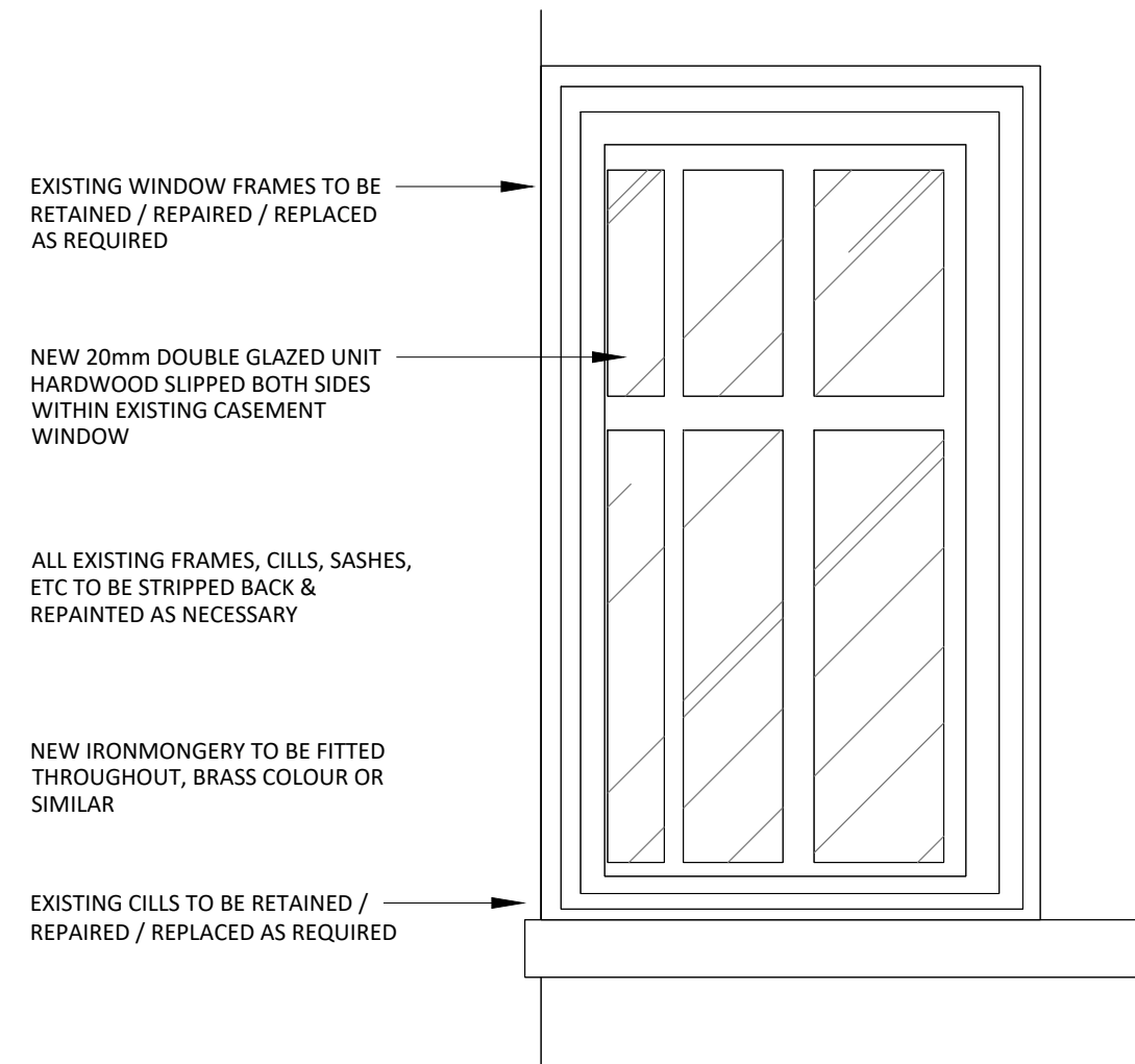
09 CURVED WINDOW PROFILE 500 ELEVATION
