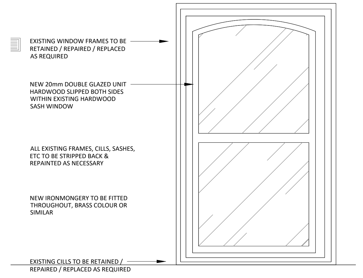
03 2ND FLOOR SASH WINDOW - TYPE B 500 ELEVATION
