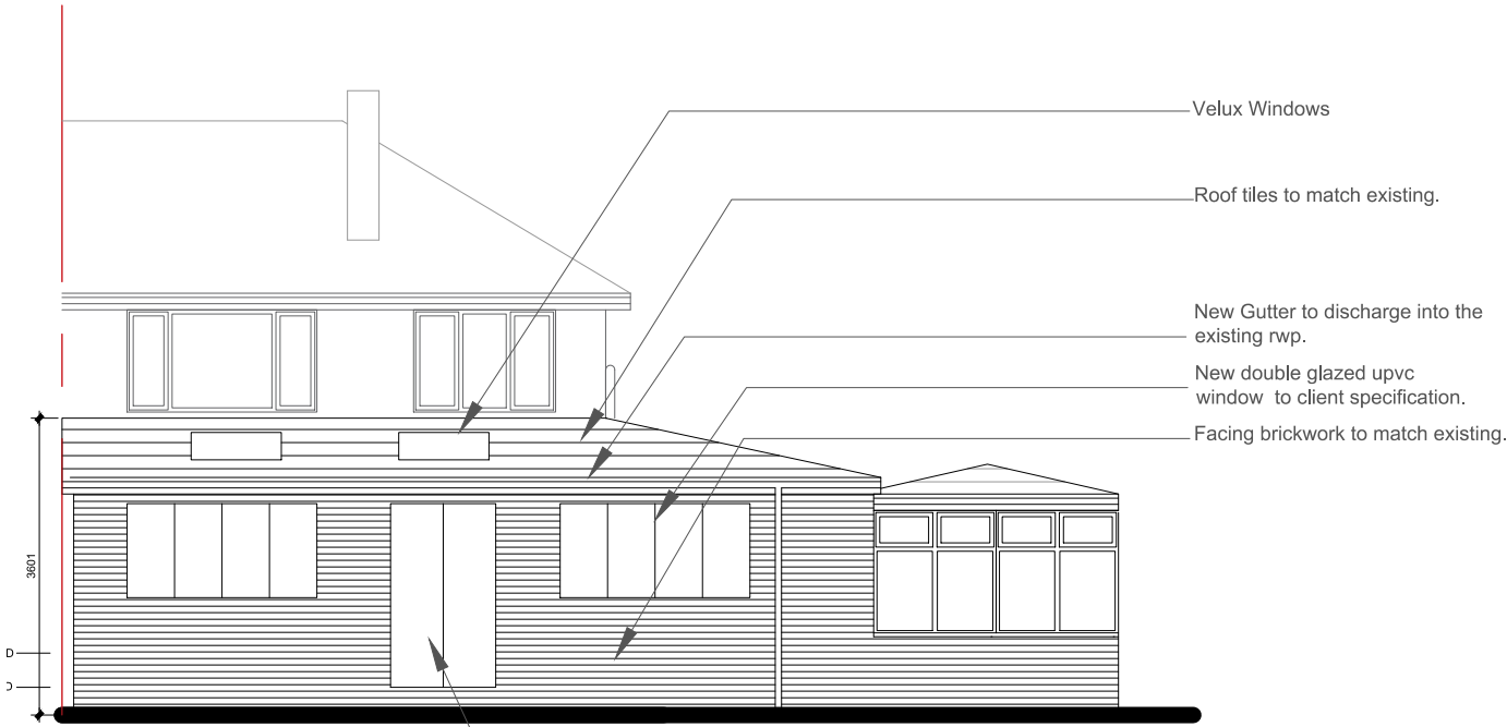
Rear Elevation
