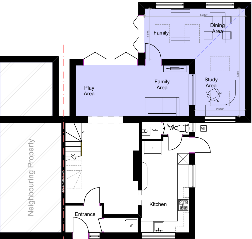
PROPOSED GA GROUND FLOOR PLAN
