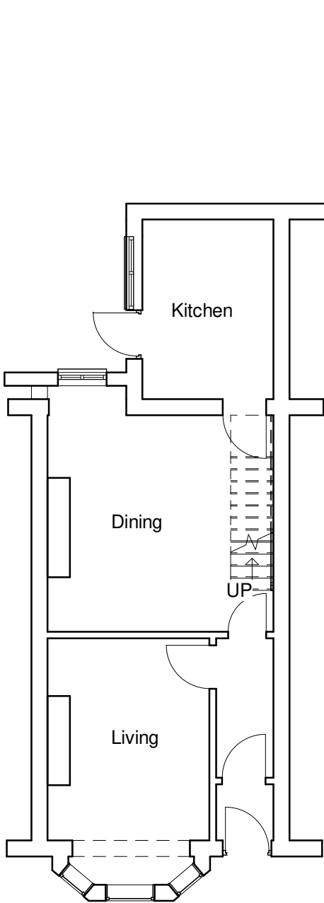
1 Ground Floor - Existing 1 : 100
