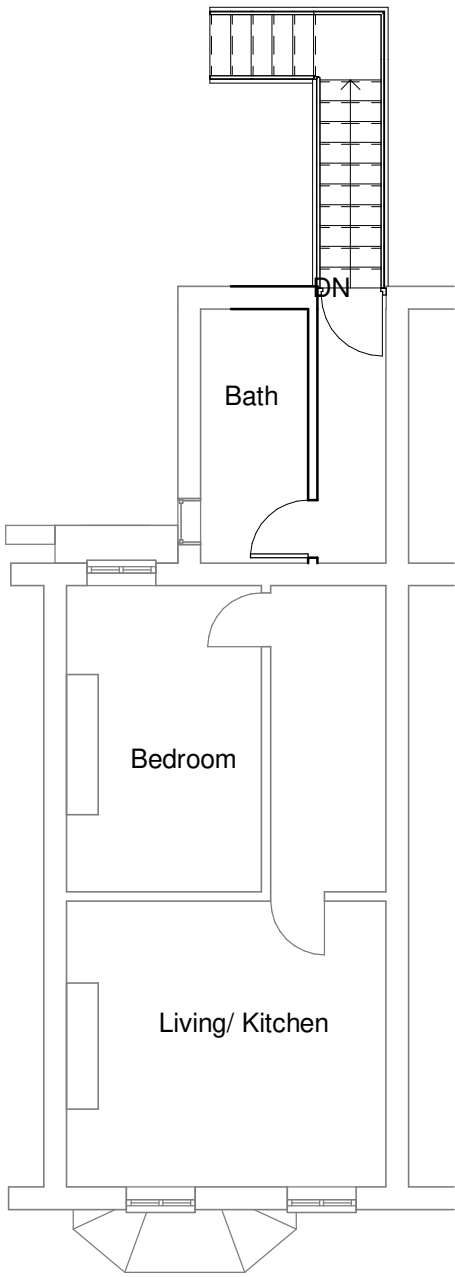
4 First Floor - Proposed 1 : 100
