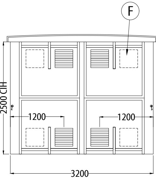
EXTERNAL VIEW ON RH WALL
