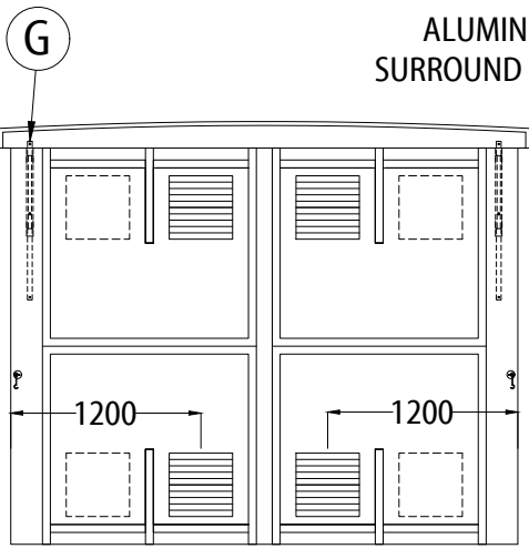
EXTERNAL VIEW ON LH WALL
