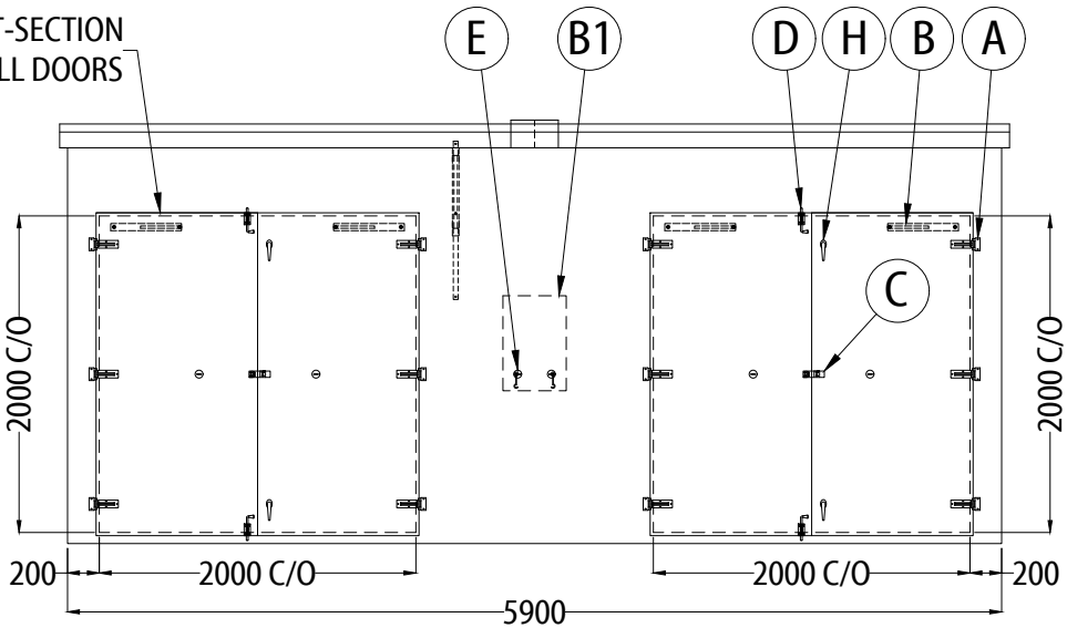
EXTERNAL VIEW ON FRONT WALL
