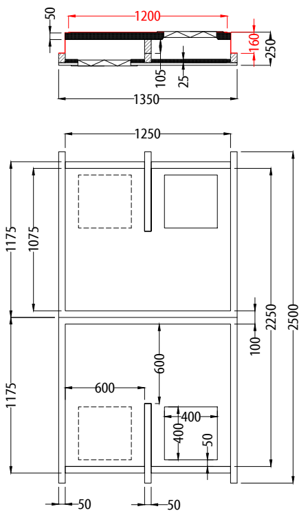
NEW ACOUSTIC BOX DETAIL
