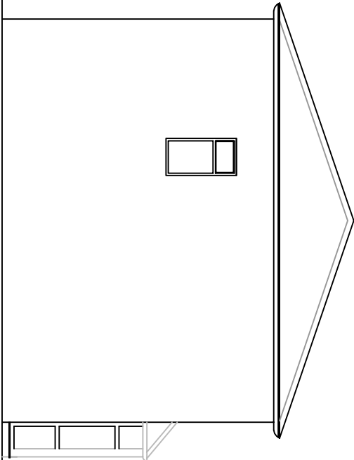
EXISTING ADJACENT SIDE ELEVATION
