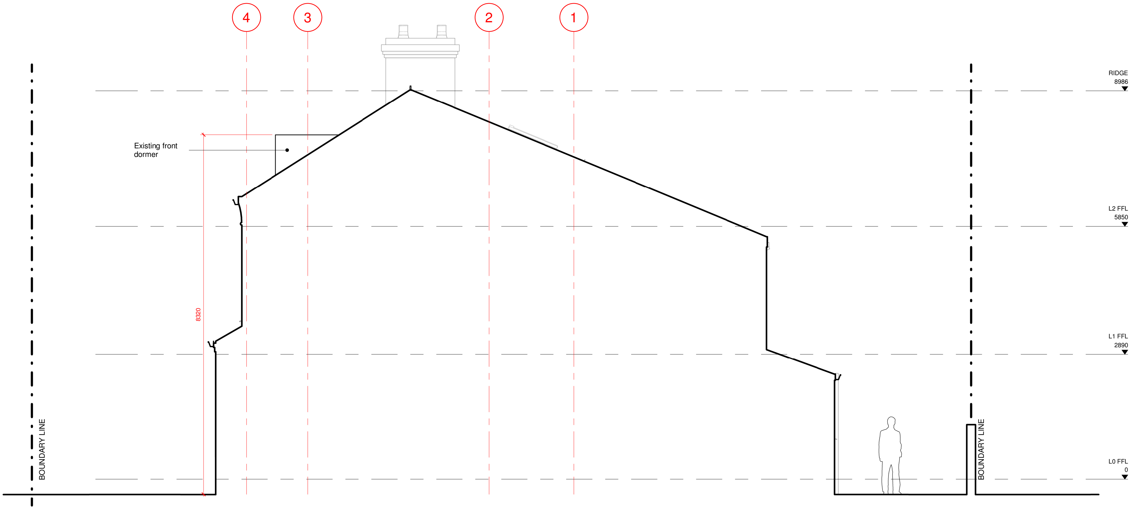
02 EXISTING RIGHT ELEVATION 1 : 50
