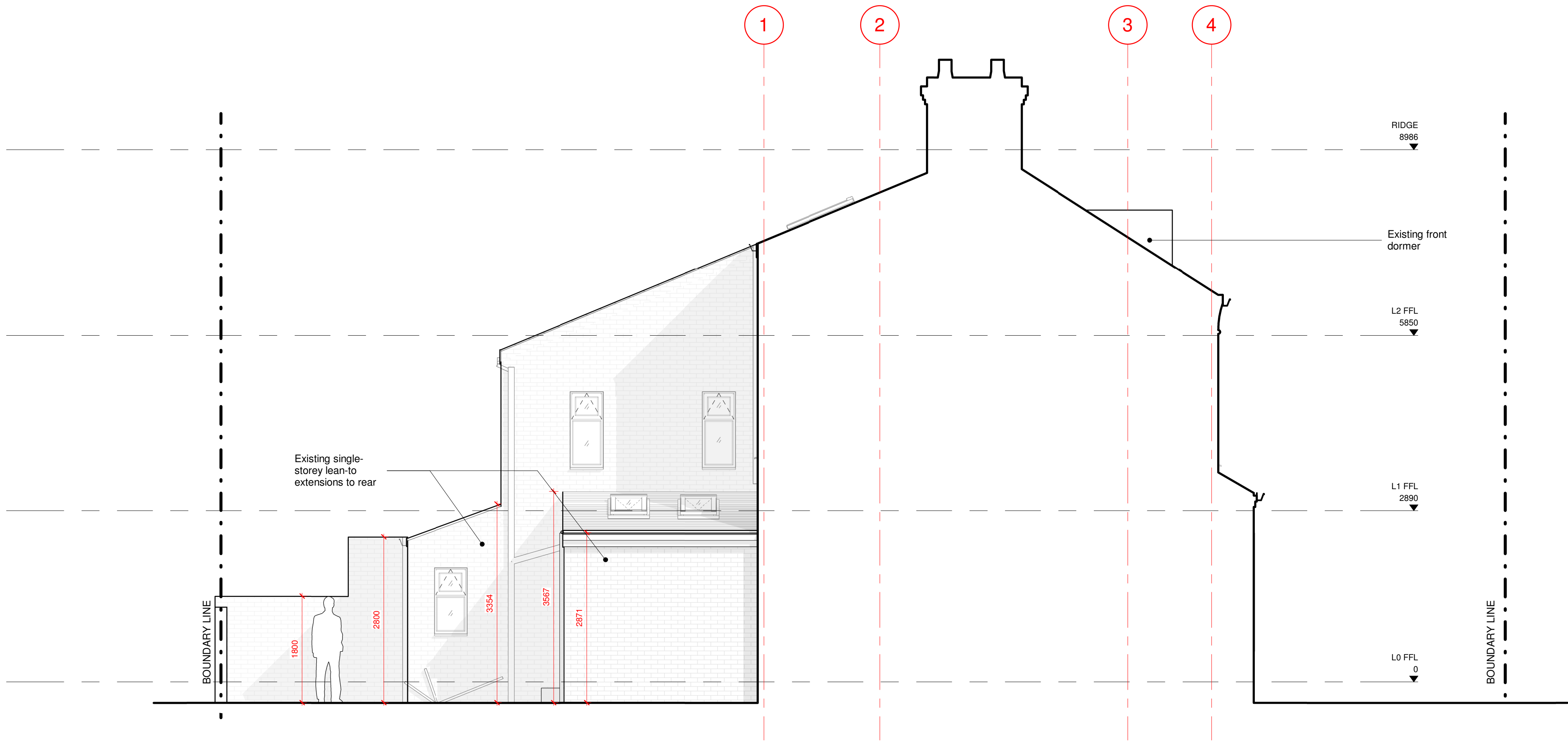
01 EXISTING LEFT ELEVATION 1 : 50
