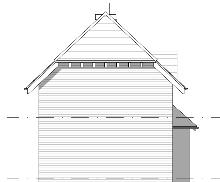
EXISTING FLANK ELEVATION 1:100
