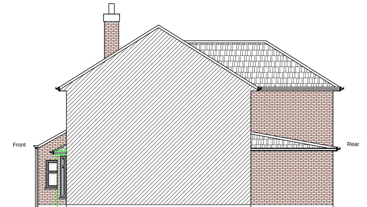
PROPOSED FLANK ELEVATION
