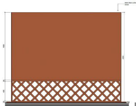
② (95) Display Board - Front Elevation 1:10
