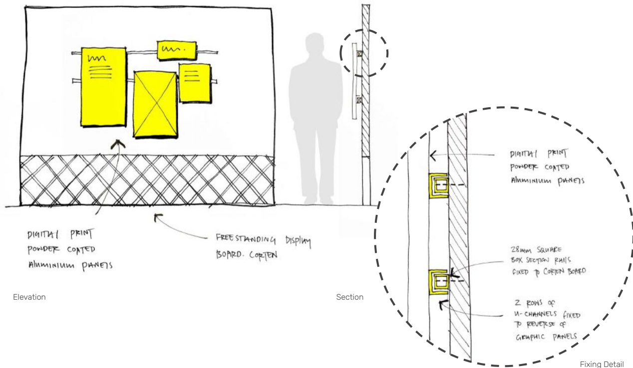
Fixing Detail
