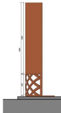
⑤ (95) Display Board - Section 1:10
