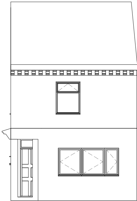
2 existing, right elevation, setout 1 : 100
