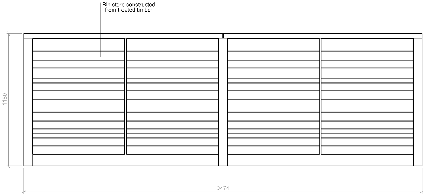
Front and rear elevations
