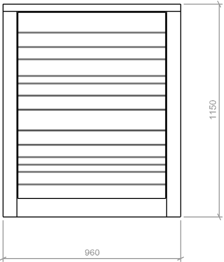
Side elevations
