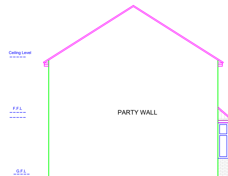
PROPOSED SIDE ELEVATION (NORTH) (NO CHANGE)
